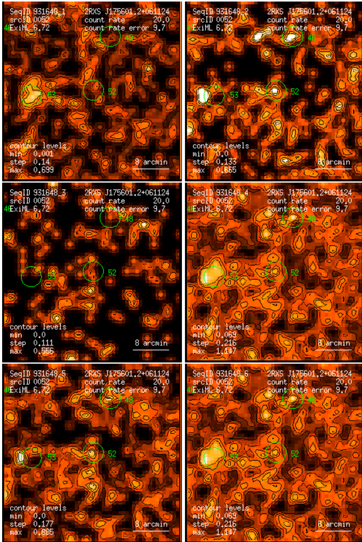
Figure 52: RASS 931648: detection 0052: band rate images, Gaussian filter: (1) PSPC channels 11 – 41, (2) 52 – 90, (3) 91 – 201, (4) 11 – 235, (5) 52 – 201, (6) 11 – 201. Broad band rates in counts/ks. Band rate contour levels in counts/ks/arcmin 2 .
