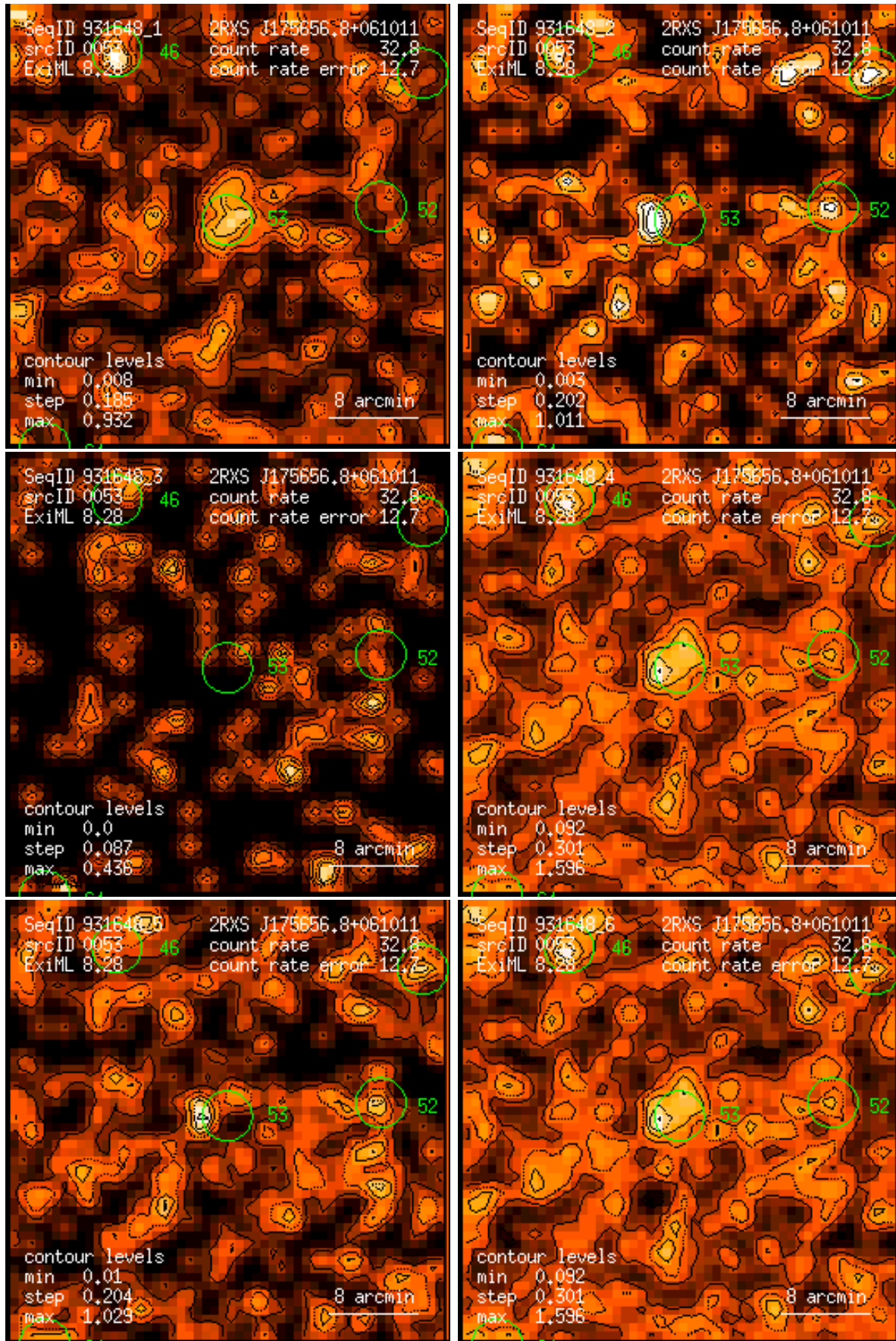
Figure 53: RASS 931648: detection 0053: band rate images, Gaussian filter: (1) PSPC channels 11 – 41, (2) 52 – 90, (3) 91 – 201, (4) 11 – 235, (5) 52 – 201, (6) 11 – 201. Broad band rates in counts/ks. Band rate contour levels in counts/ks/arcmin 2 .
