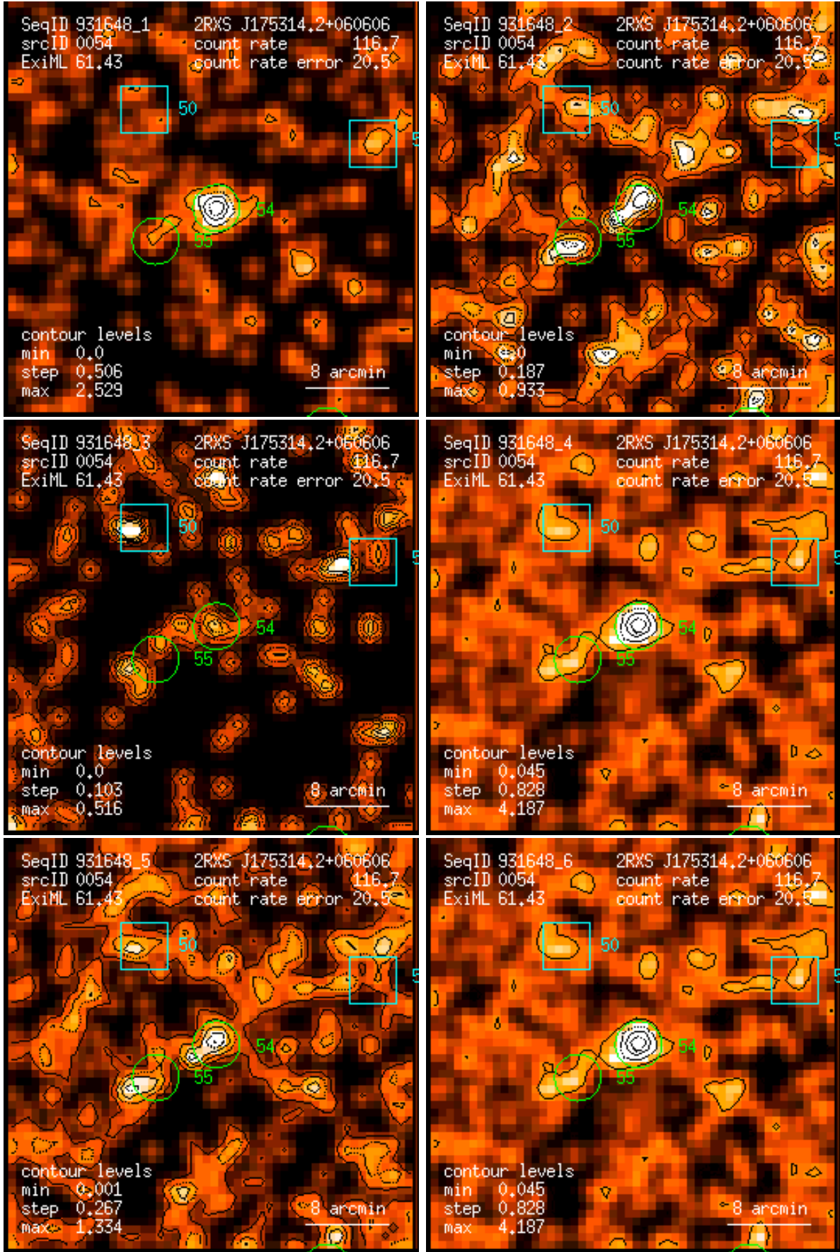
Figure 54: RASS 931648: detection 0054: band rate images, Gaussian filter: (1) PSPC channels 11 – 41, (2) 52 – 90, (3) 91 – 201, (4) 11 – 235, (5) 52 – 201, (6) 11 – 201. Broad band rates in counts/ks. Band rate contour levels in counts/ks/arcmin 2 .
