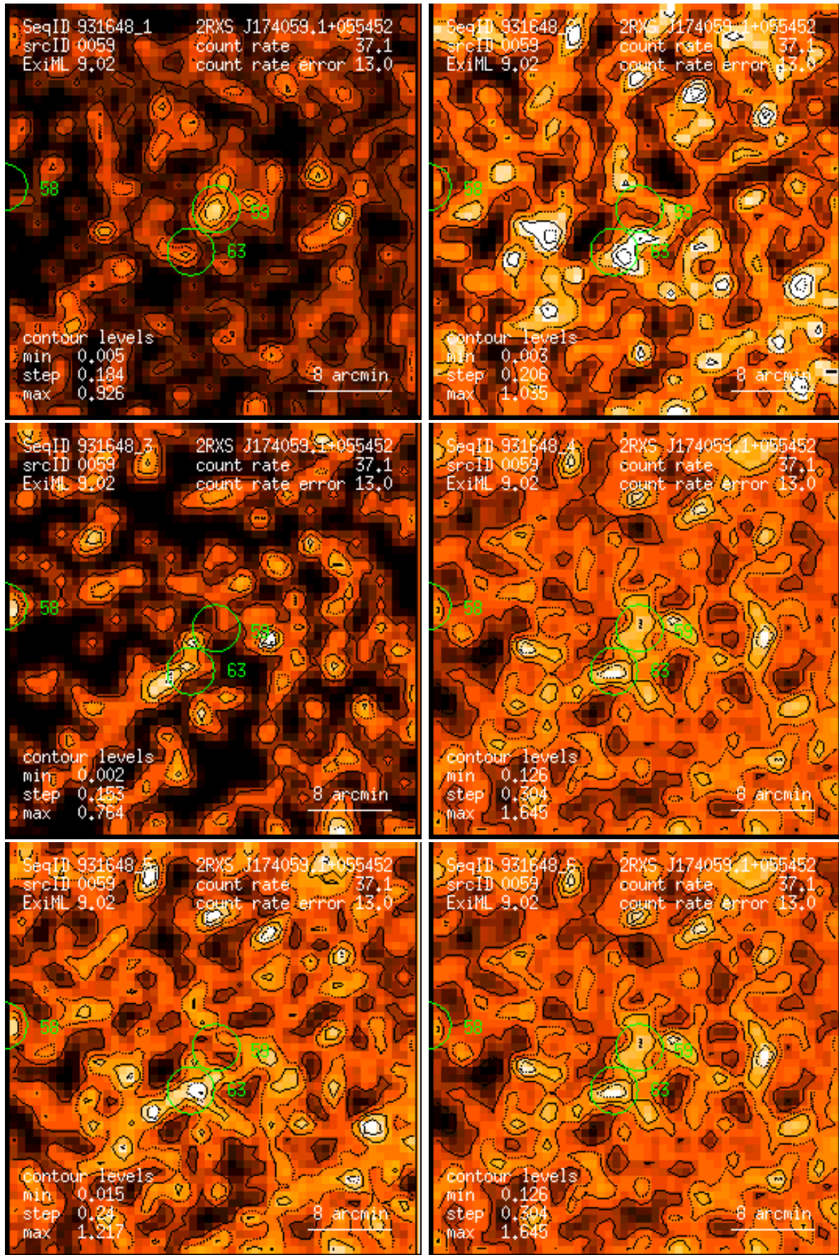
Figure 59: RASS 931648: detection 0059: band rate images, Gaussian filter: (1) PSPC channels 11 – 41, (2) 52 – 90, (3) 91 – 201, (4) 11 – 235, (5) 52 – 201, (6) 11 – 201. Broad band rates in counts/ks. Band rate contour levels in counts/ks/arcmin 2 .
