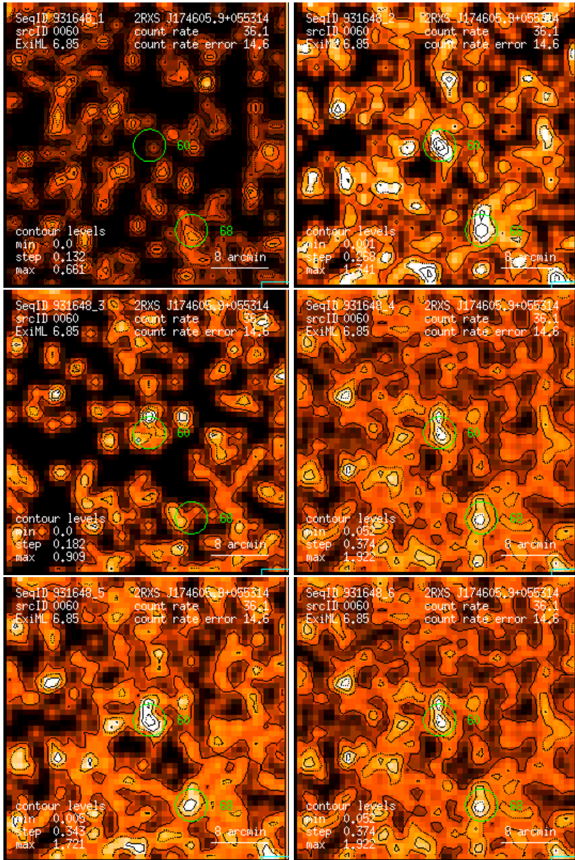
Figure 60: RASS 931648: detection 0060: band rate images, Gaussian filter: (1) PSPC channels 11 – 41, (2) 52 – 90, (3) 91 – 201, (4) 11 – 235, (5) 52 – 201, (6) 11 – 201. Broad band rates in counts/ks. Band rate contour levels in counts/ks/arcmin 2 .
