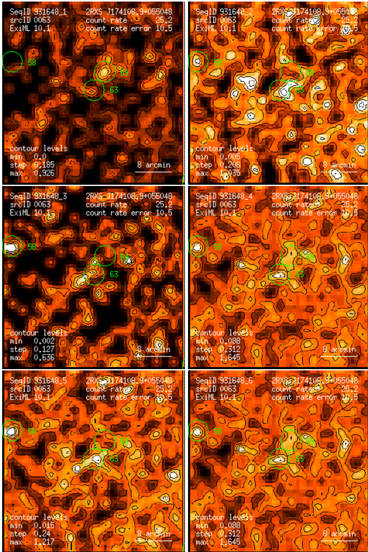
Figure 63: RASS 931648: detection 0063: band rate images, Gaussian filter: (1) PSPC channels 11 – 41, (2) 52 – 90, (3) 91 – 201, (4) 11 – 235, (5) 52 – 201, (6) 11 – 201. Broad band rates in counts/ks. Band rate contour levels in counts/ks/arcmin 2 .
