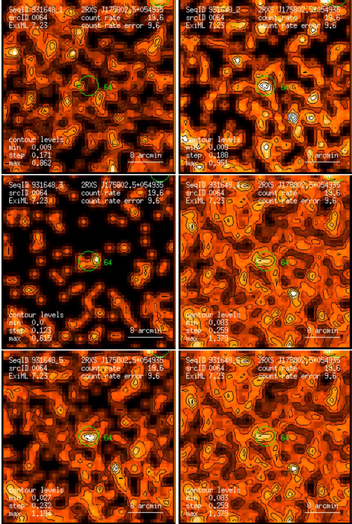
Figure 64: RASS 931648: detection 0064: band rate images, Gaussian filter: (1) PSPC channels 11 – 41, (2) 52 – 90, (3) 91 – 201, (4) 11 – 235, (5) 52 – 201, (6) 11 – 201. Broad band rates in counts/ks. Band rate contour levels in counts/ks/arcmin 2 .
