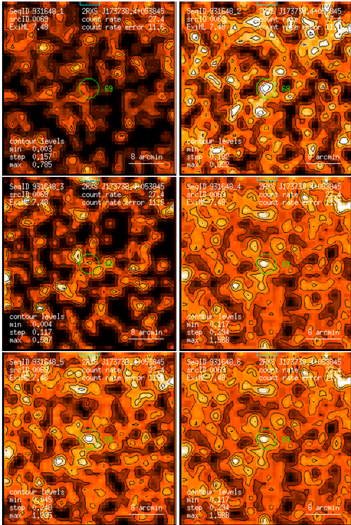
Figure 69: RASS 931648: detection 0069: band rate images, Gaussian filter: (1) PSPC channels 11 – 41, (2) 52 – 90, (3) 91 – 201, (4) 11 – 235, (5) 52 – 201, (6) 11 – 201. Broad band rates in counts/ks. Band rate contour levels in counts/ks/arcmin 2 .
