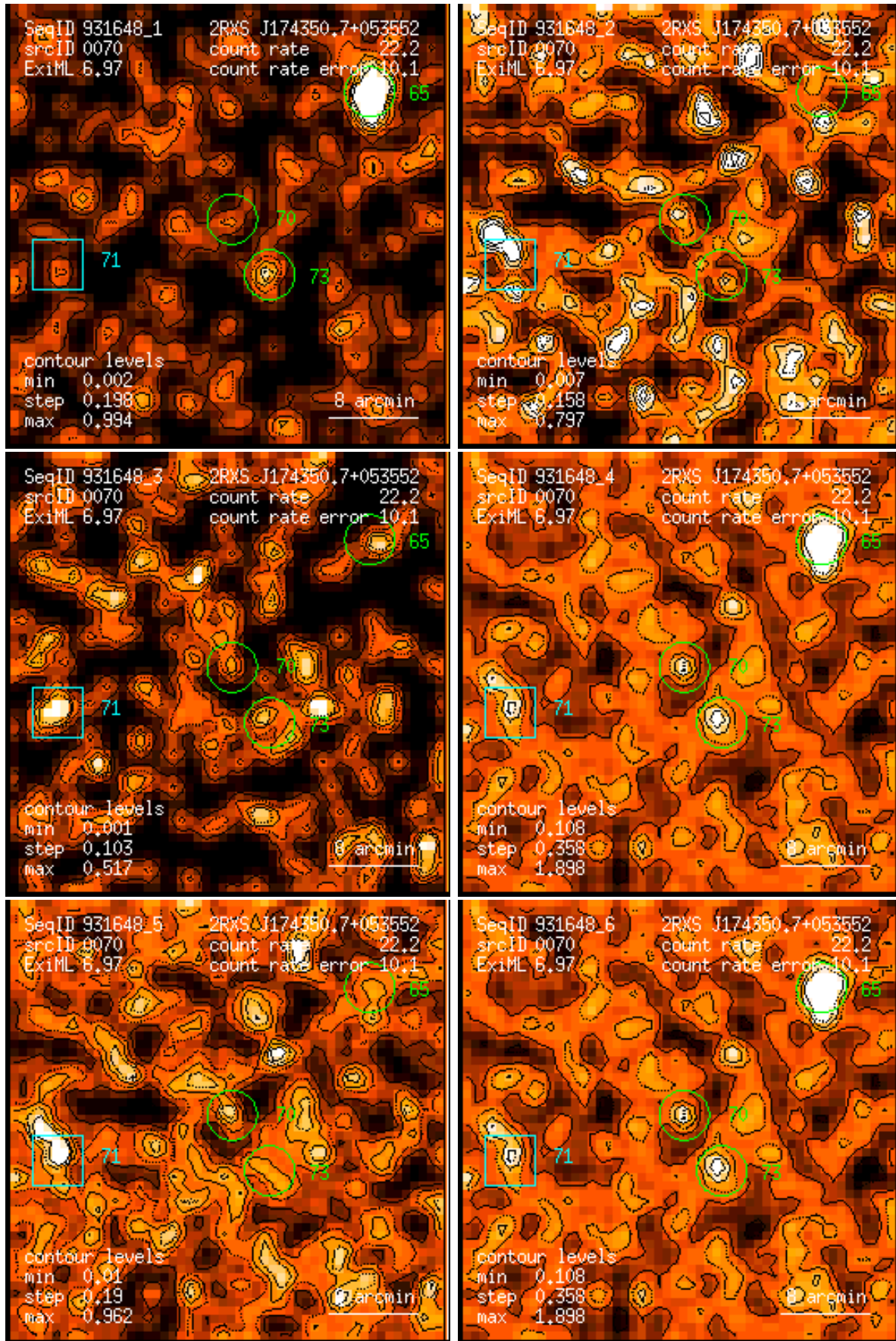
Figure 70: RASS 931648: detection 0070: band rate images, Gaussian filter: (1) PSPC channels 11 – 41, (2) 52 – 90, (3) 91 – 201, (4) 11 – 235, (5) 52 – 201, (6) 11 – 201. Broad band rates in counts/ks. Band rate contour levels in counts/ks/arcmin 2 .
