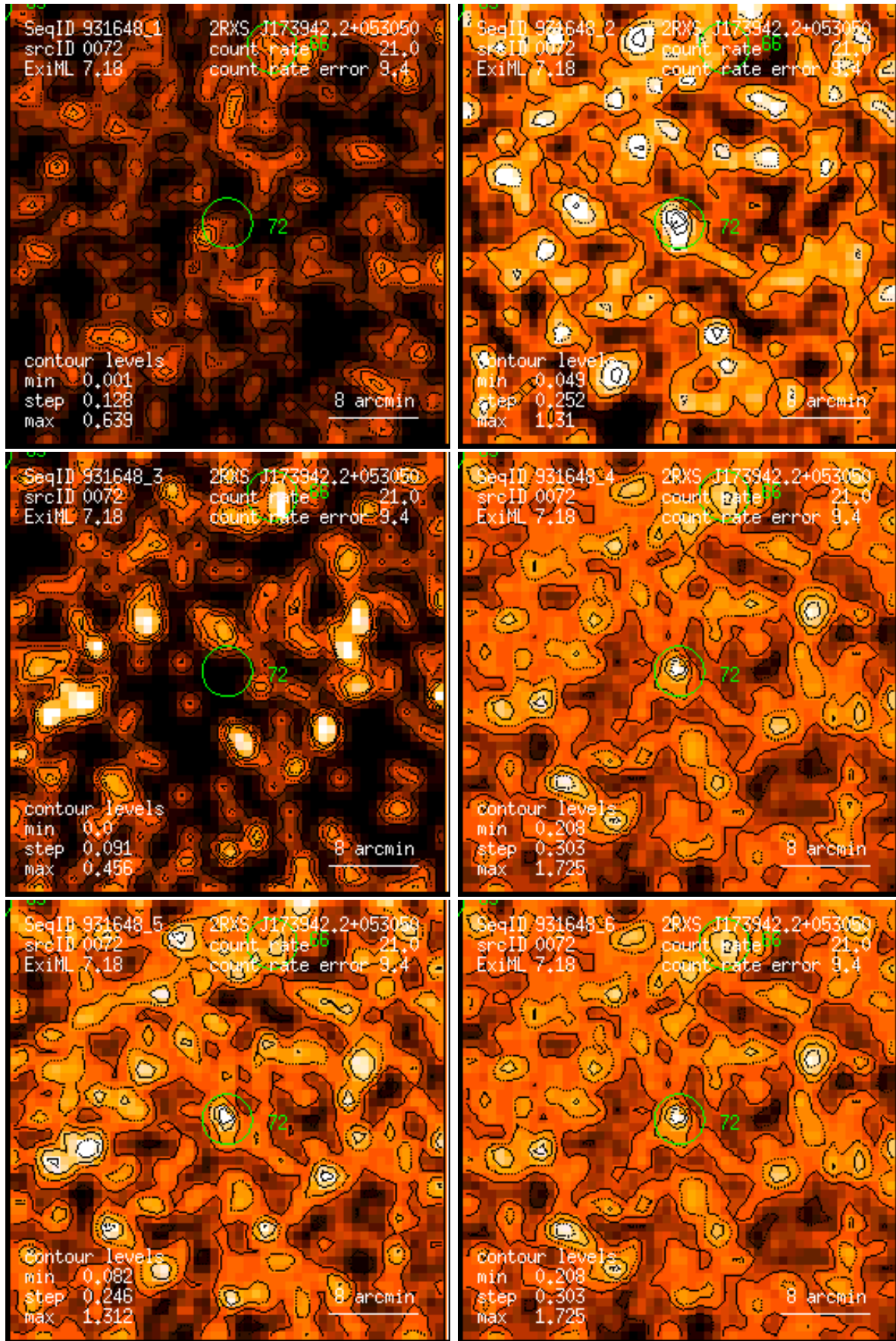
Figure 72: RASS 931648: detection 0072: band rate images, Gaussian filter: (1) PSPC channels 11 – 41, (2) 52 – 90, (3) 91 – 201, (4) 11 – 235, (5) 52 – 201, (6) 11 – 201. Broad band rates in counts/ks. Band rate contour levels in counts/ks/arcmin 2 .
