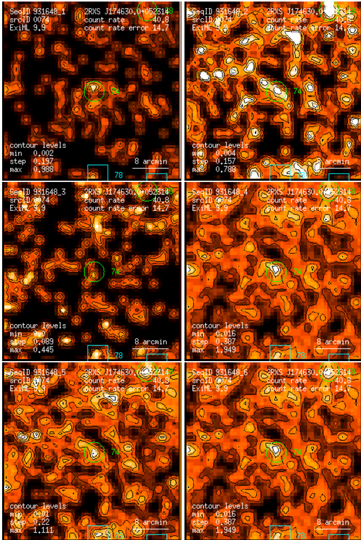
Figure 74: RASS 931648: detection 0074: band rate images, Gaussian filter: (1) PSPC channels 11 – 41, (2) 52 – 90, (3) 91 – 201, (4) 11 – 235, (5) 52 – 201, (6) 11 – 201. Broad band rates in counts/ks. Band rate contour levels in counts/ks/arcmin 2 .
