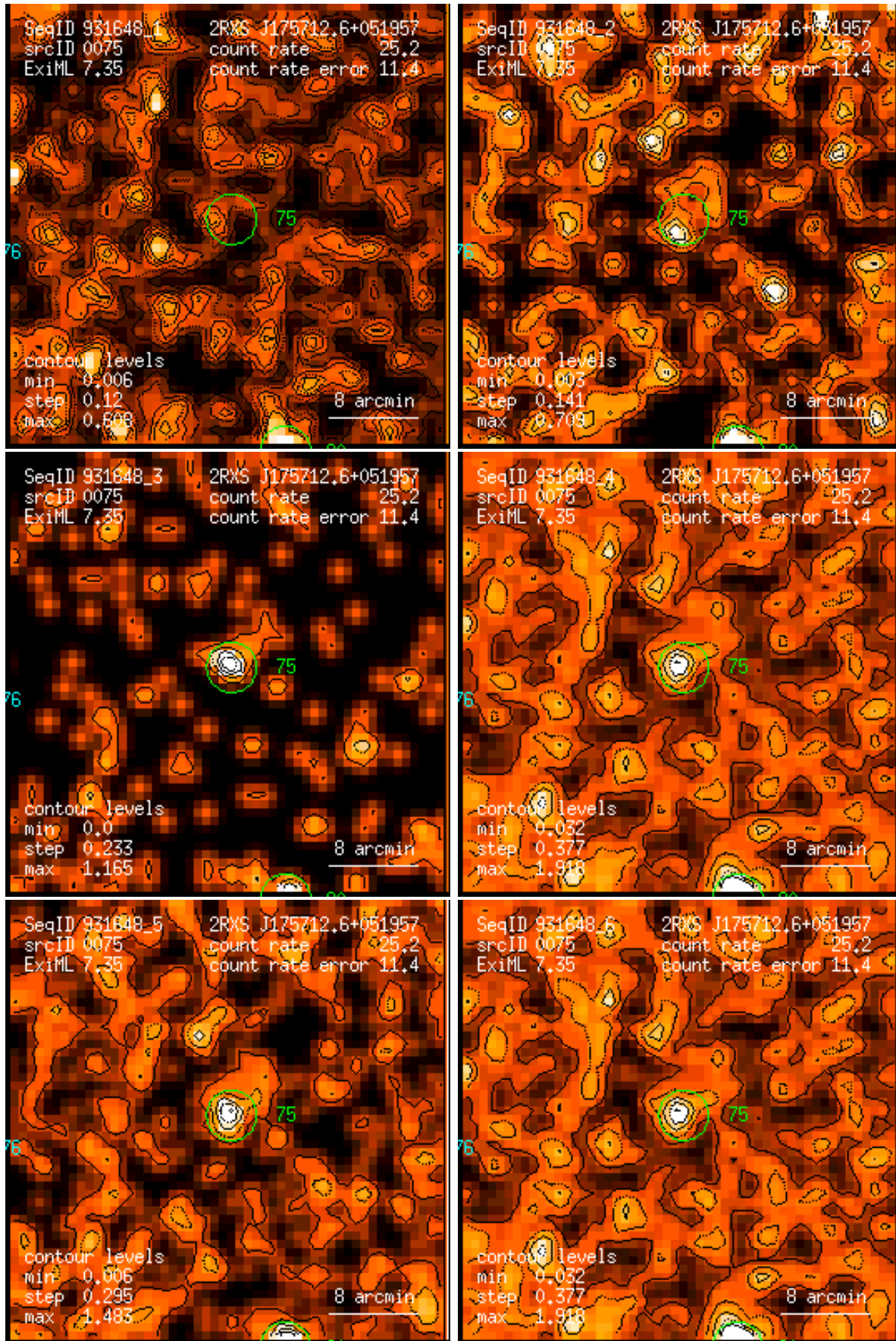
Figure 75: RASS 931648: detection 0075: band rate images, Gaussian filter: (1) PSPC channels 11 – 41, (2) 52 – 90, (3) 91 – 201, (4) 11 – 235, (5) 52 – 201, (6) 11 – 201. Broad band rates in counts/ks. Band rate contour levels in counts/ks/arcmin 2 .
