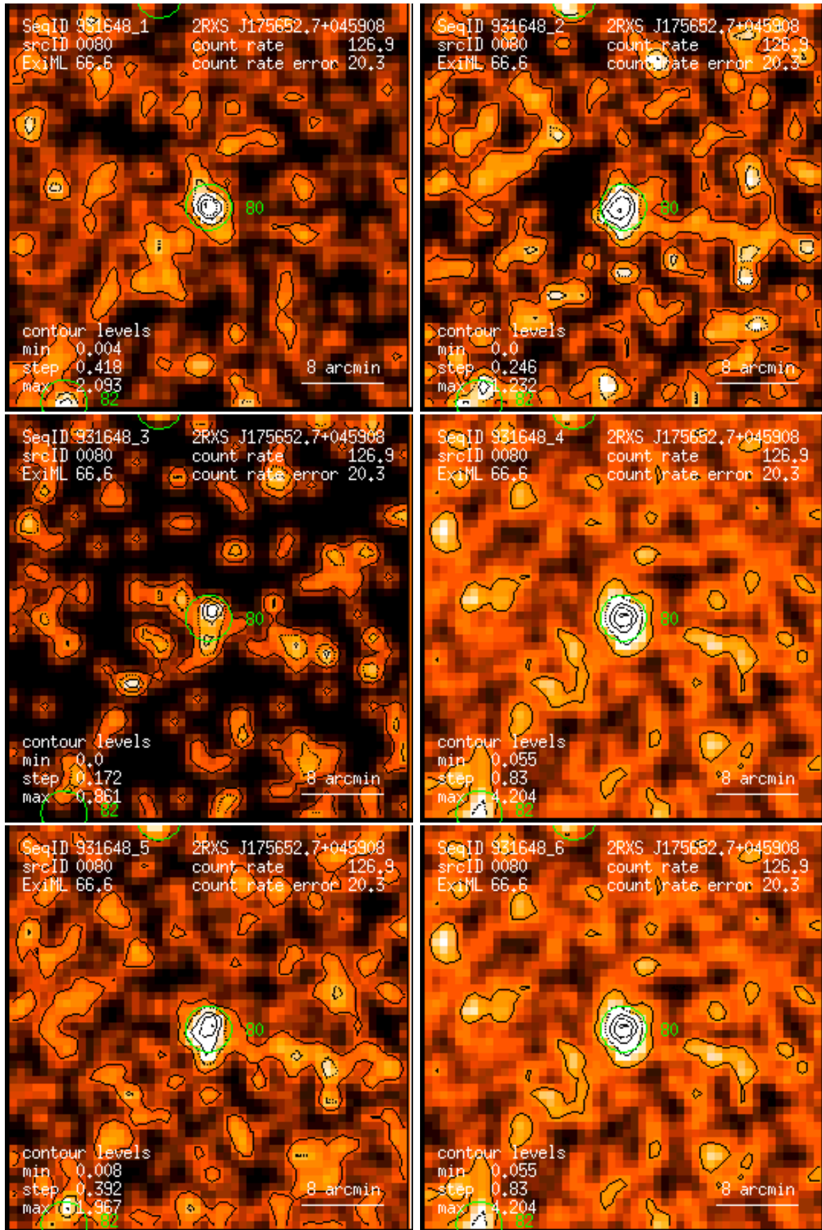
Figure 80: RASS 931648: detection 0080: band rate images, Gaussian filter: (1) PSPC channels 11 – 41, (2) 52 – 90, (3) 91 – 201, (4) 11 – 235, (5) 52 – 201, (6) 11 – 201. Broad band rates in counts/ks. Band rate contour levels in counts/ks/arcmin 2 .
