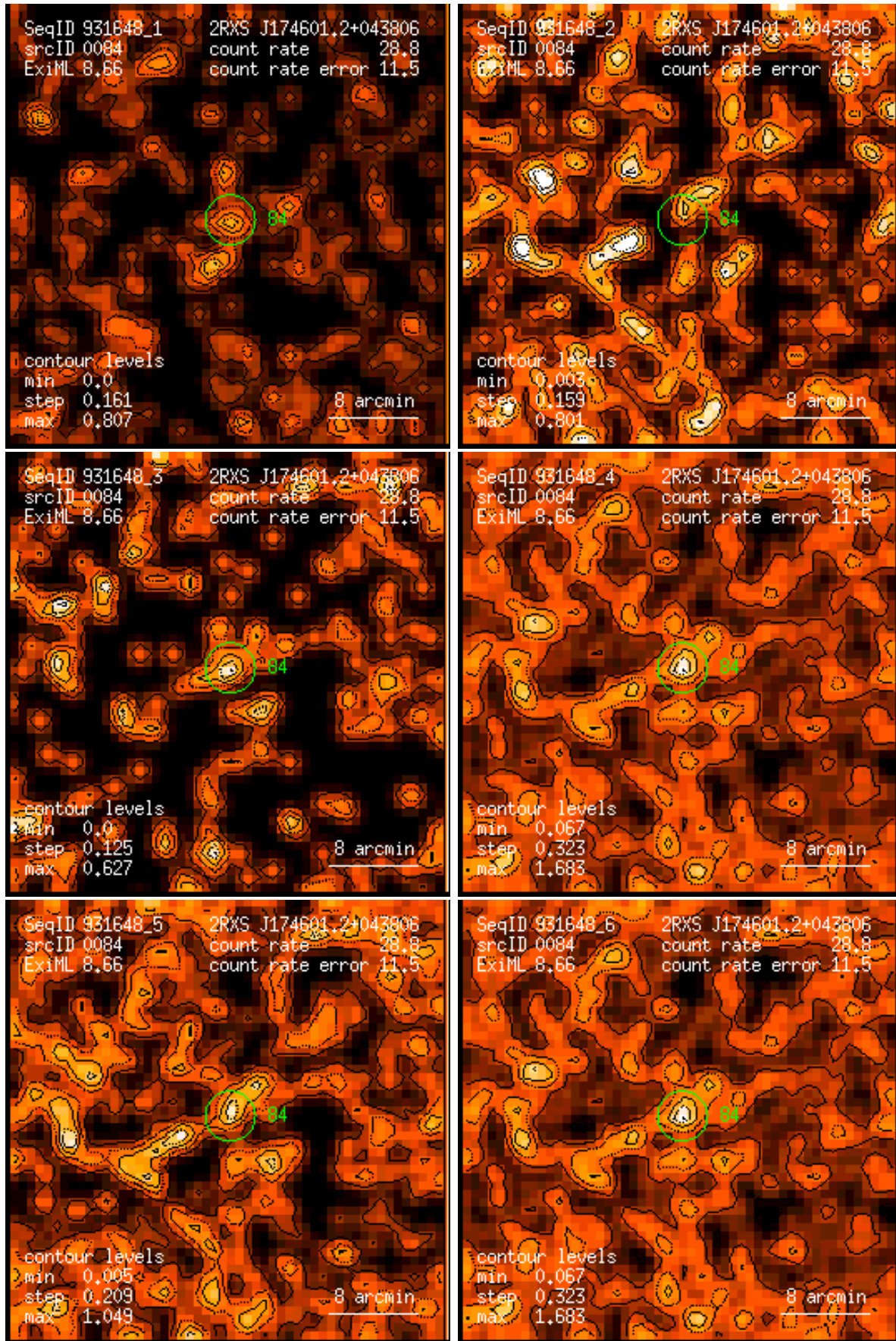
Figure 84: RASS 931648: detection 0084: band rate images, Gaussian filter: (1) PSPC channels 11 – 41, (2) 52 – 90, (3) 91 – 201, (4) 11 – 235, (5) 52 – 201, (6) 11 – 201. Broad band rates in counts/ks. Band rate contour levels in counts/ks/arcmin 2 .
