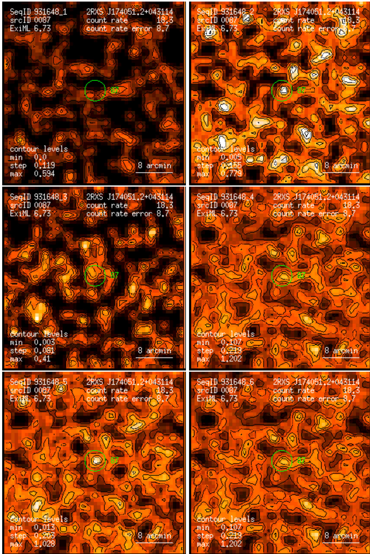
Figure 87: RASS 931648: detection 0087: band rate images, Gaussian filter: (1) PSPC channels 11 – 41, (2) 52 – 90, (3) 91 – 201, (4) 11 – 235, (5) 52 – 201, (6) 11 – 201. Broad band rates in counts/ks. Band rate contour levels in counts/ks/arcmin 2 .
