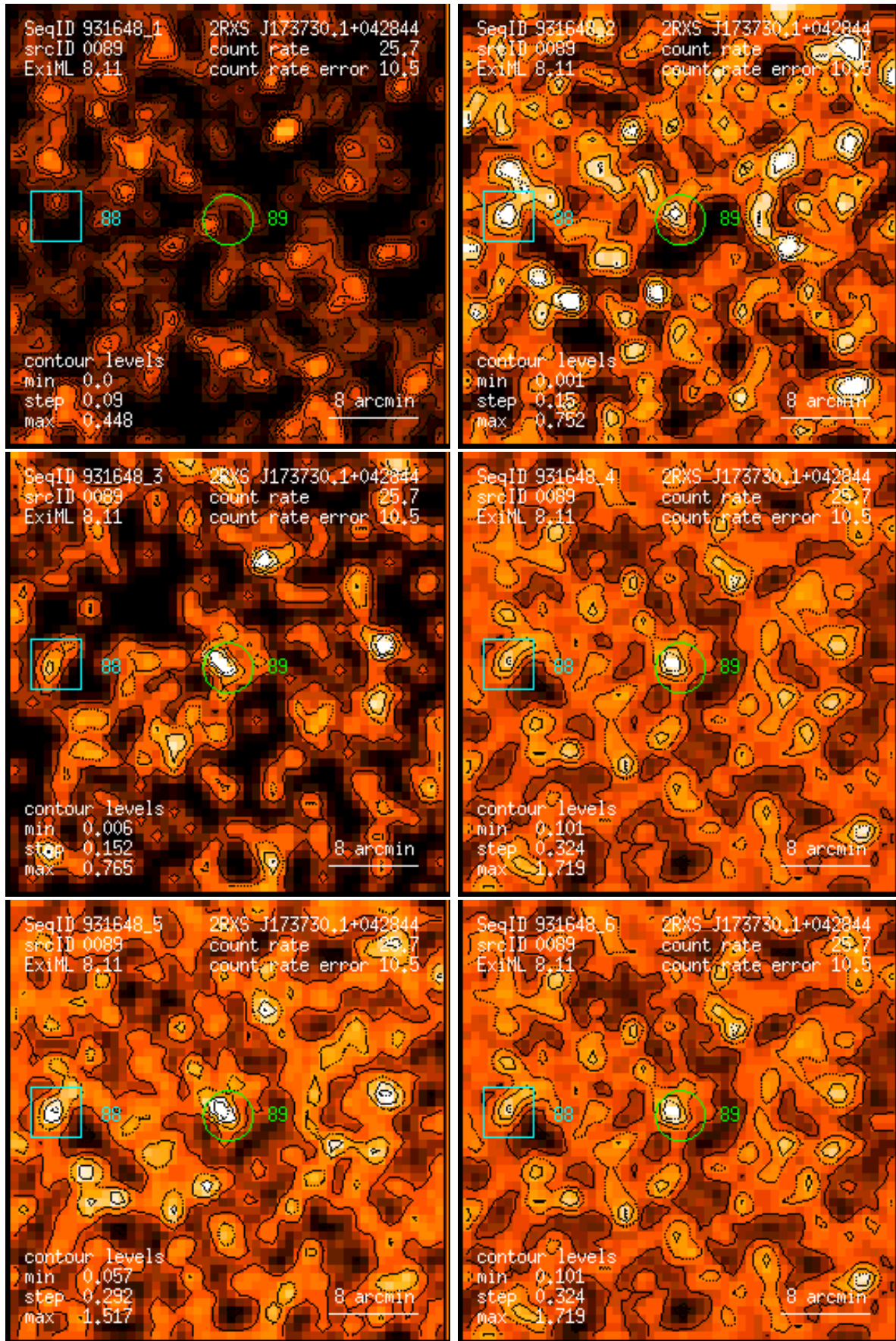
Figure 89: RASS 931648: detection 0089: band rate images, Gaussian filter: (1) PSPC channels 11 – 41, (2) 52 – 90, (3) 91 – 201, (4) 11 – 235, (5) 52 – 201, (6) 11 – 201. Broad band rates in counts/ks. Band rate contour levels in counts/ks/arcmin 2 .
