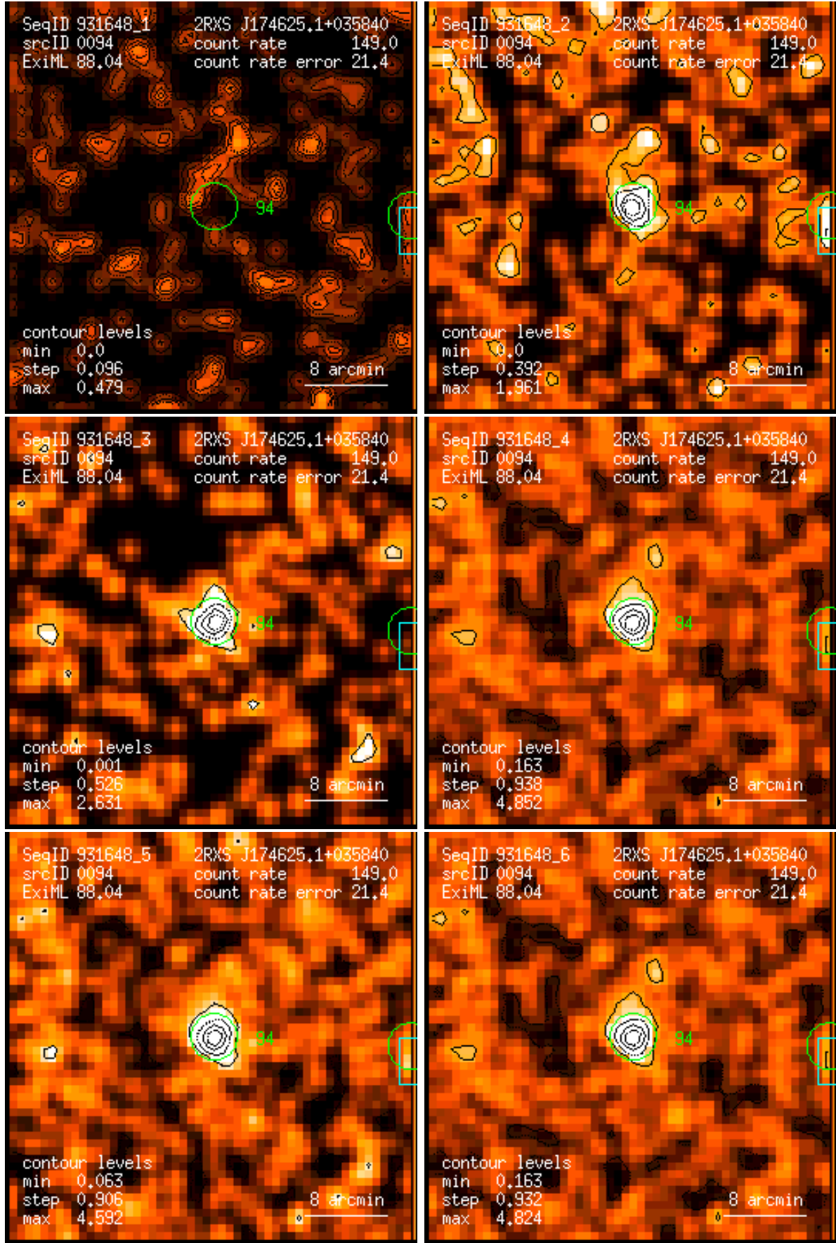
Figure 94: RASS 931648: detection 0094: band rate images, Gaussian filter: (1) PSPC channels 11 – 41, (2) 52 – 90, (3) 91 – 201, (4) 11 – 235, (5) 52 – 201, (6) 11 – 201. Broad band rates in counts/ks. Band rate contour levels in counts/ks/arcmin 2 .
