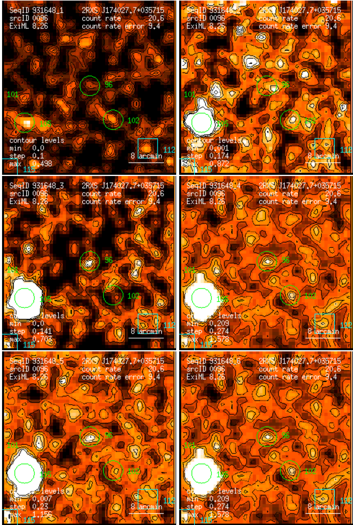
Figure 96: RASS 931648: detection 0096: band rate images, Gaussian filter: (1) PSPC channels 11 – 41, (2) 52 – 90, (3) 91 – 201, (4) 11 – 235, (5) 52 – 201, (6) 11 – 201. Broad band rates in counts/ks. Band rate contour levels in counts/ks/arcmin 2 .
