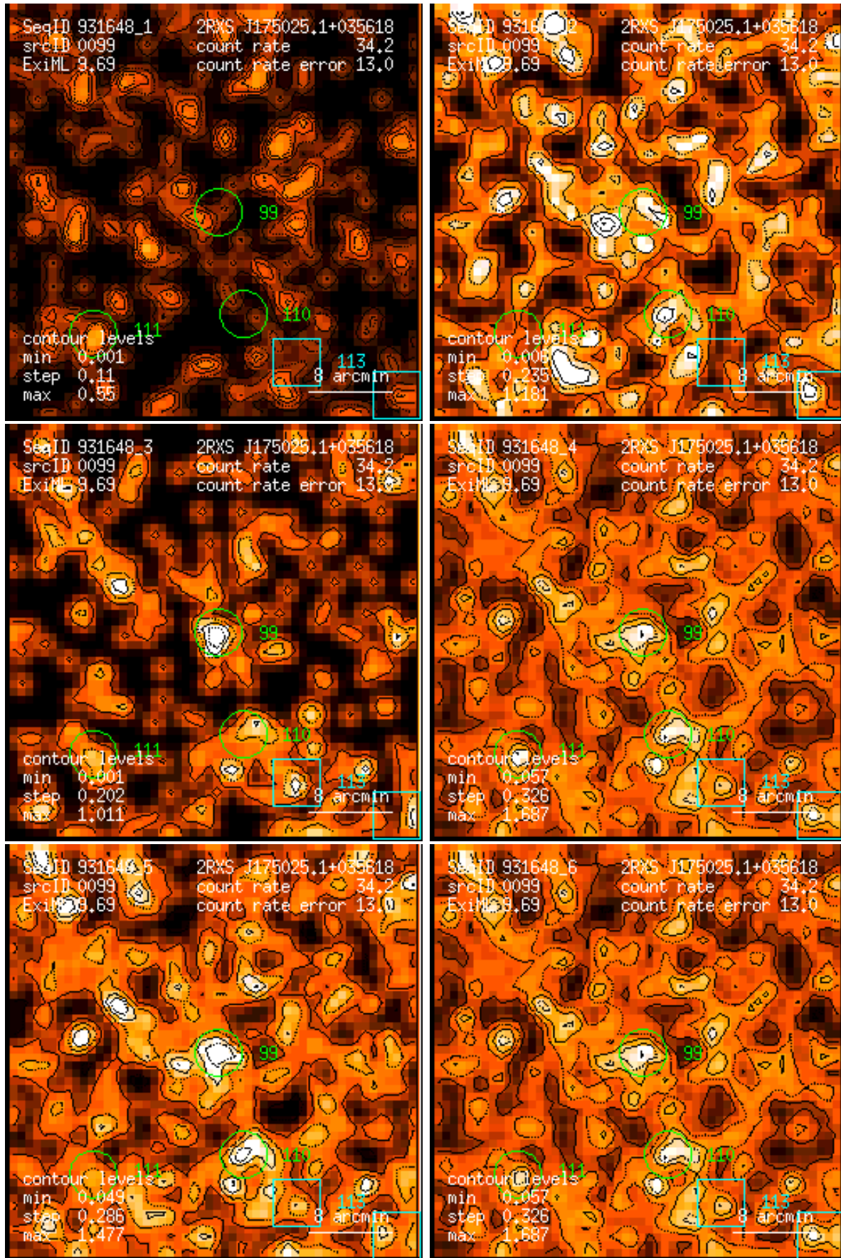
Figure 99: RASS 931648: detection 0099: band rate images, Gaussian filter: (1) PSPC channels 11 – 41, (2) 52 – 90, (3) 91 – 201, (4) 11 – 235, (5) 52 – 201, (6) 11 – 201. Broad band rates in counts/ks. Band rate contour levels in counts/ks/arcmin 2 .
