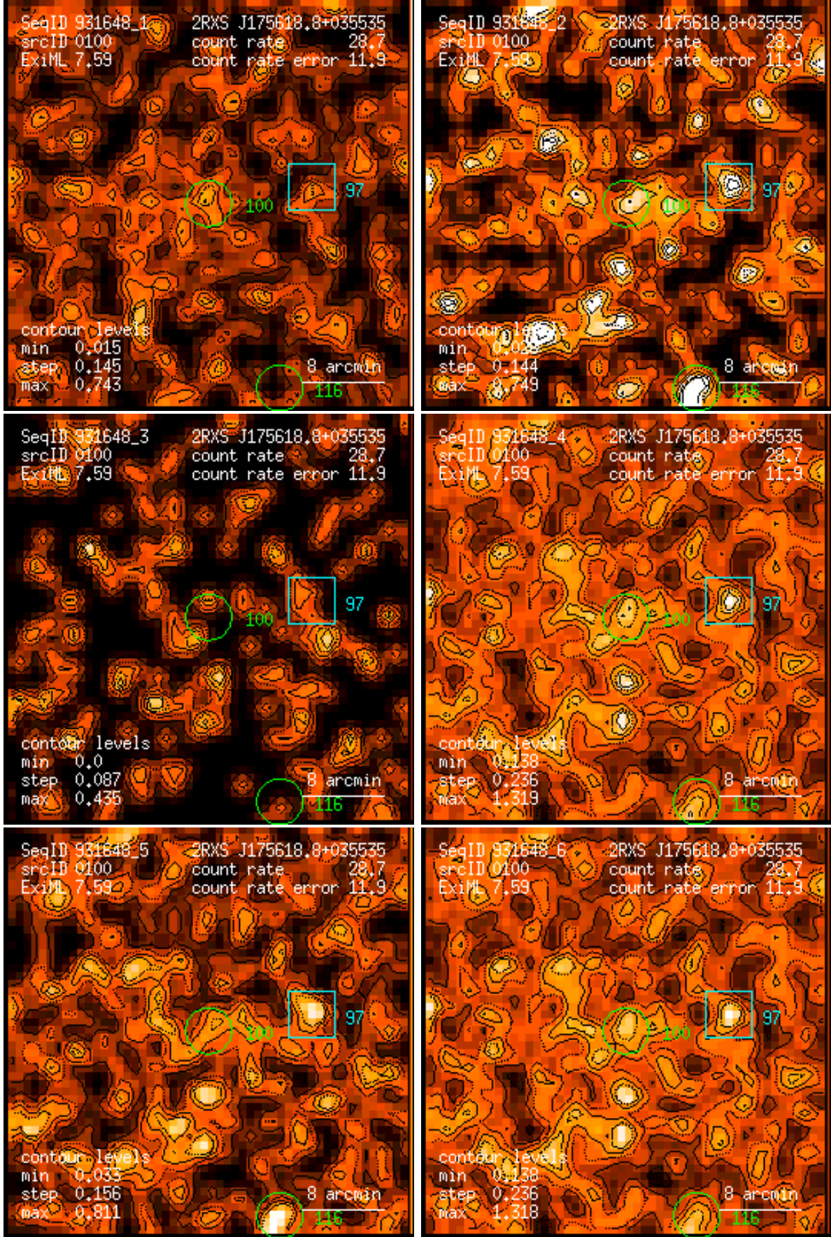
Figure 100: RASS 931648: detection 0100: band rate images, Gaussian filter: (1) PSPC channels 11 – 41, (2) 52 – 90, (3) 91 – 201, (4) 11 – 235, (5) 52 – 201, (6) 11 – 201. Broad band rates in counts/ks. Band rate contour levels in counts/ks/arcmin 2 .
