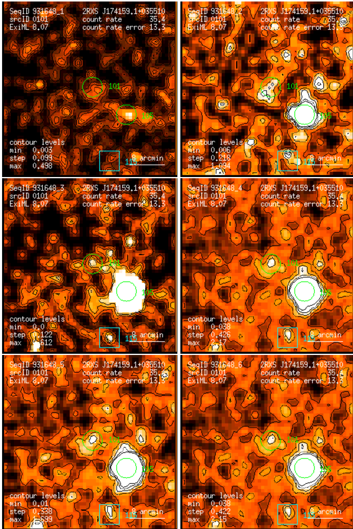
Figure 101: RASS 931648: detection 0101: band rate images, Gaussian filter: (1) PSPC channels 11 – 41, (2) 52 – 90, (3) 91 – 201, (4) 11 – 235, (5) 52 – 201, (6) 11 – 201. Broad band rates in counts/ks. Band rate contour levels in counts/ks/arcmin 2 .
