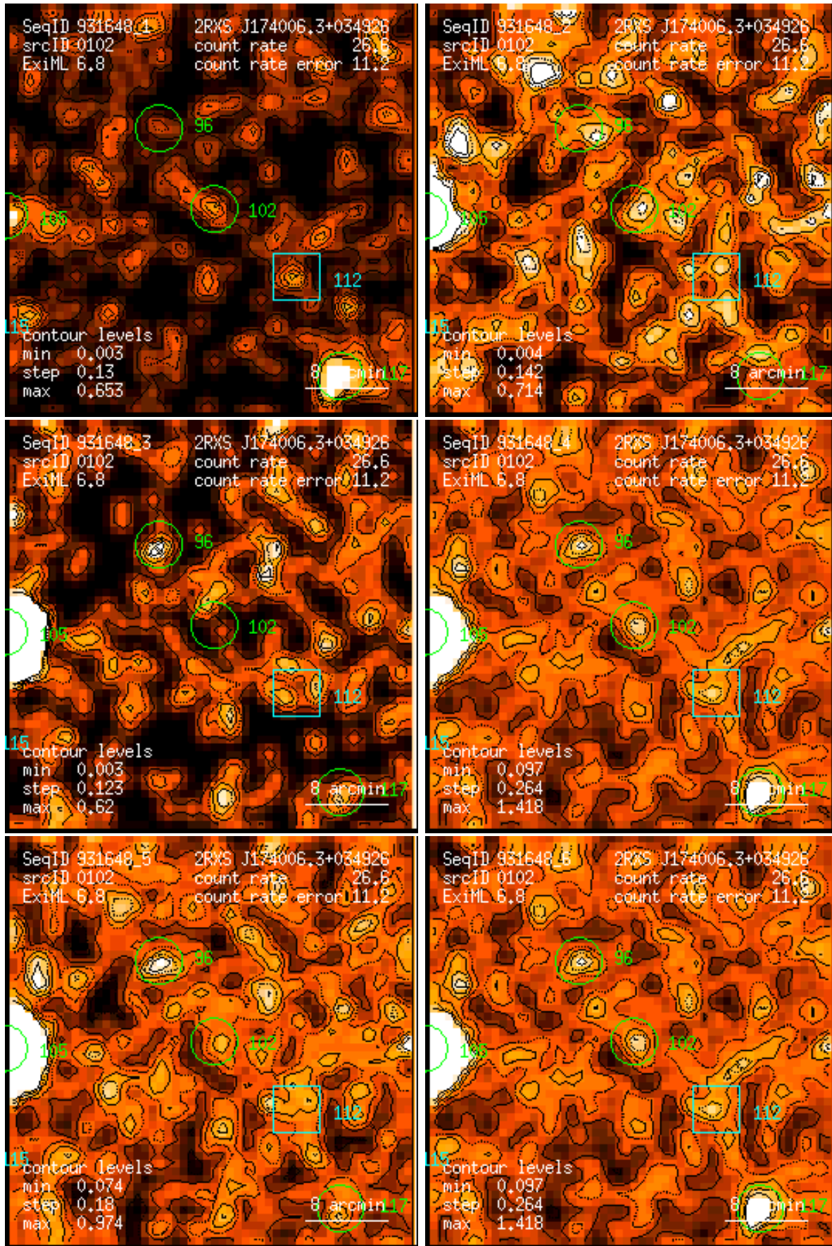
Figure 102: RASS 931648: detection 0102: band rate images, Gaussian filter: (1) PSPC channels 11 – 41, (2) 52 – 90, (3) 91 – 201, (4) 11 – 235, (5) 52 – 201, (6) 11 – 201. Broad band rates in counts/ks. Band rate contour levels in counts/ks/arcmin 2 .
