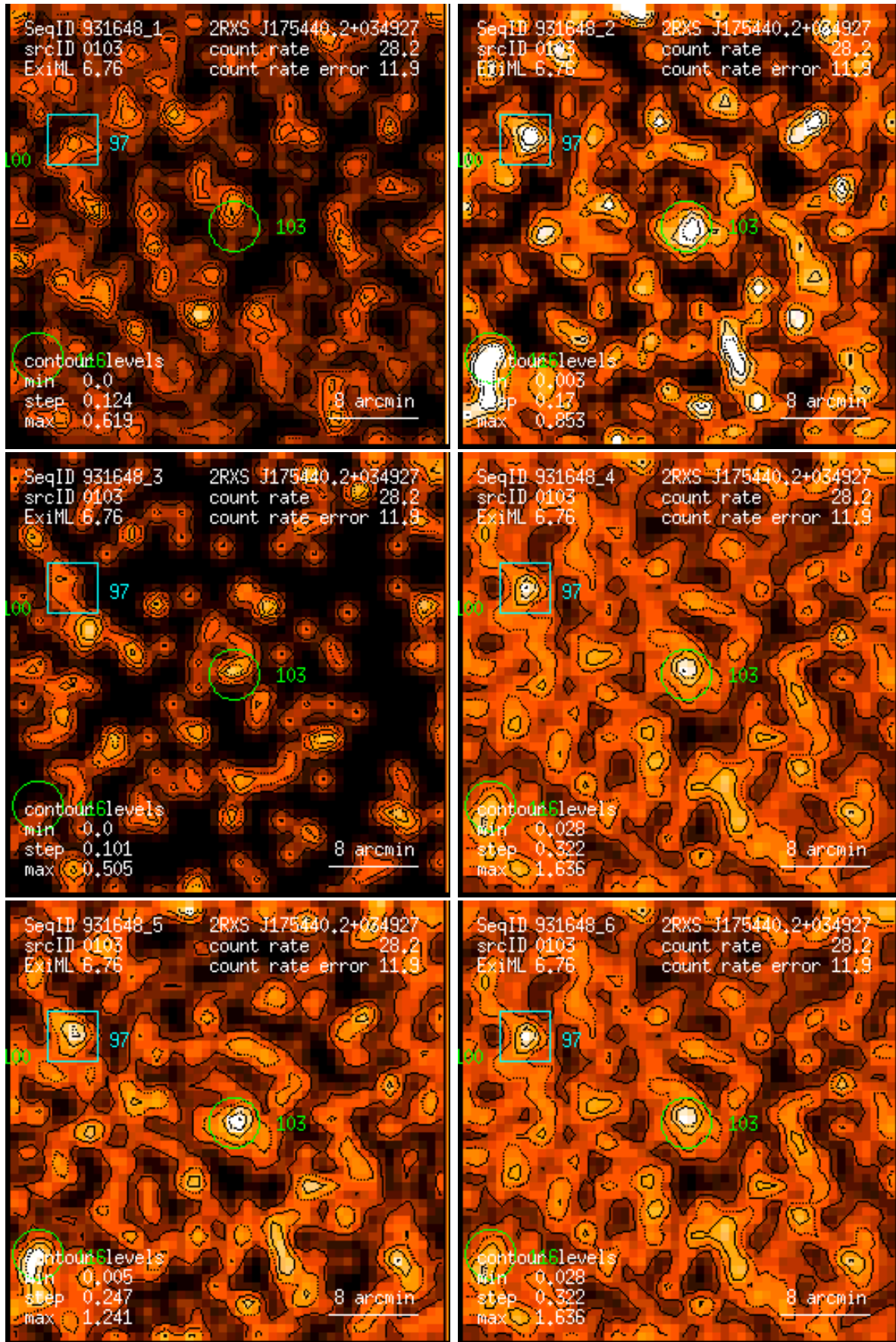
Figure 103: RASS 931648: detection 0103: band rate images, Gaussian filter: (1) PSPC channels 11 – 41, (2) 52 – 90, (3) 91 – 201, (4) 11 – 235, (5) 52 – 201, (6) 11 – 201. Broad band rates in counts/ks. Band rate contour levels in counts/ks/arcmin 2 .
