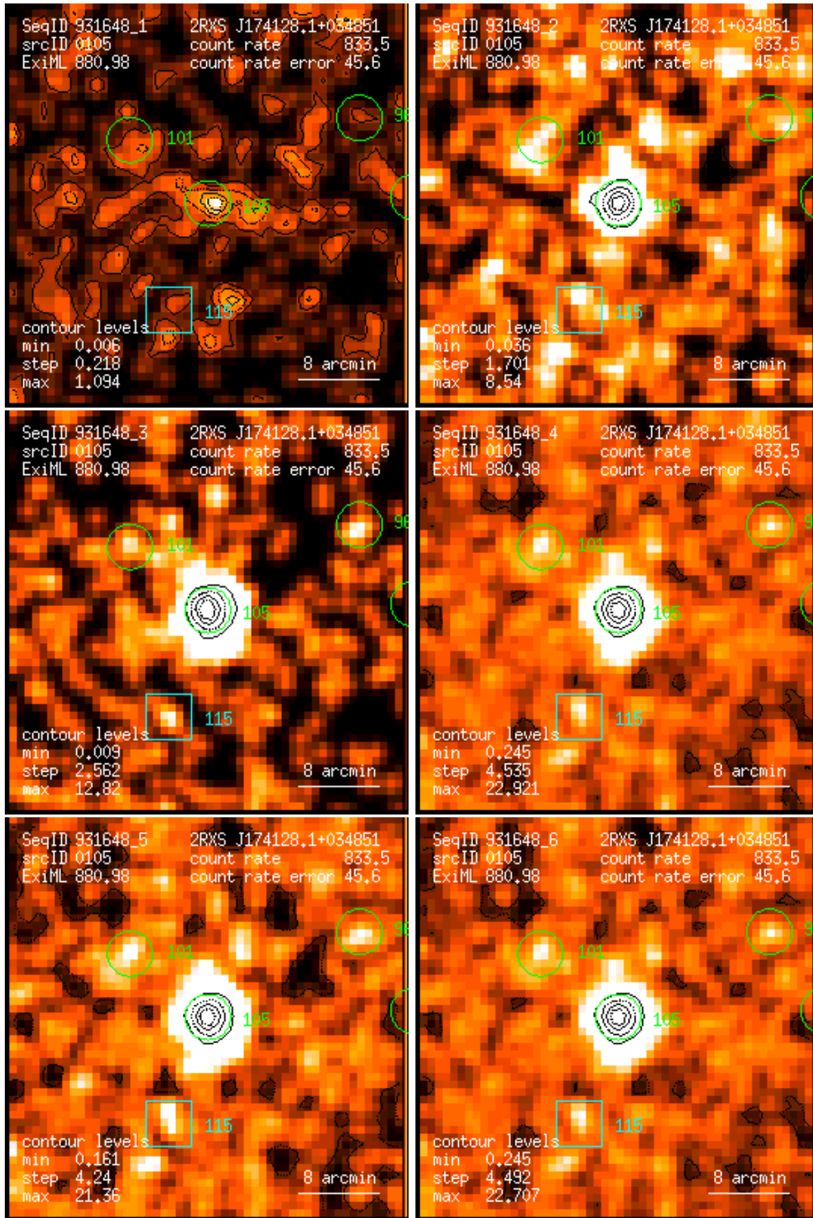
Figure 105: RASS 931648: detection 0105: band rate images, Gaussian filter: (1) PSPC channels 11 – 41, (2) 52 – 90, (3) 91 – 201, (4) 11 – 235, (5) 52 – 201, (6) 11 – 201. Broad band rates in counts/ks. Band rate contour levels in counts/ks/arcmin 2 .
