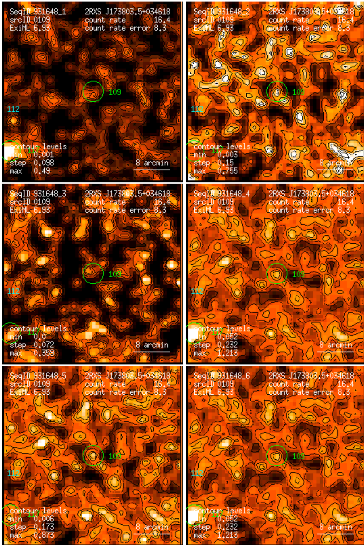
Figure 109: RASS 931648: detection 0109: band rate images, Gaussian filter: (1) PSPC channels 11 – 41, (2) 52 – 90, (3) 91 – 201, (4) 11 – 235, (5) 52 – 201, (6) 11 – 201. Broad band rates in counts/ks. Band rate contour levels in counts/ks/arcmin 2 .
