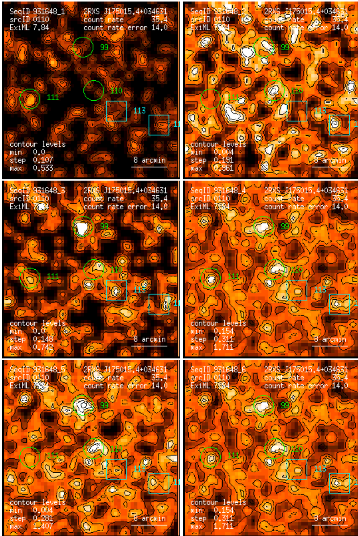
Figure 110: RASS 931648: detection 0110: band rate images, Gaussian filter: (1) PSPC channels 11 – 41, (2) 52 – 90, (3) 91 – 201, (4) 11 – 235, (5) 52 – 201, (6) 11 – 201. Broad band rates in counts/ks. Band rate contour levels in counts/ks/arcmin 2 .
