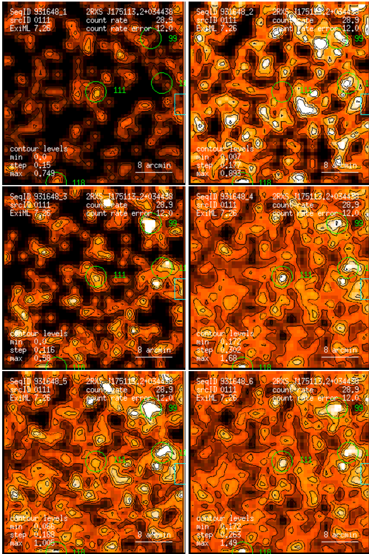
Figure 111: RASS 931648: detection 0111: band rate images, Gaussian filter: (1) PSPC channels 11 – 41, (2) 52 – 90, (3) 91 – 201, (4) 11 – 235, (5) 52 – 201, (6) 11 – 201. Broad band rates in counts/ks. Band rate contour levels in counts/ks/arcmin 2 .
