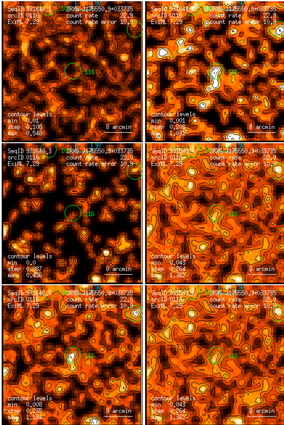
Figure 116: RASS 931648: detection 0116: band rate images, Gaussian filter: (1) PSPC channels 11 – 41, (2) 52 – 90, (3) 91 – 201, (4) 11 – 235, (5) 52 – 201, (6) 11 – 201. Broad band rates in counts/ks. Band rate contour levels in counts/ks/arcmin 2 .
