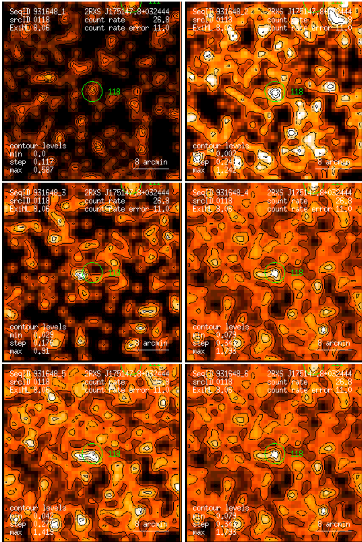
Figure 118: RASS 931648: detection 0118: band rate images, Gaussian filter: (1) PSPC channels 11 – 41, (2) 52 – 90, (3) 91 – 201, (4) 11 – 235, (5) 52 – 201, (6) 11 – 201. Broad band rates in counts/ks. Band rate contour levels in counts/ks/arcmin 2 .
