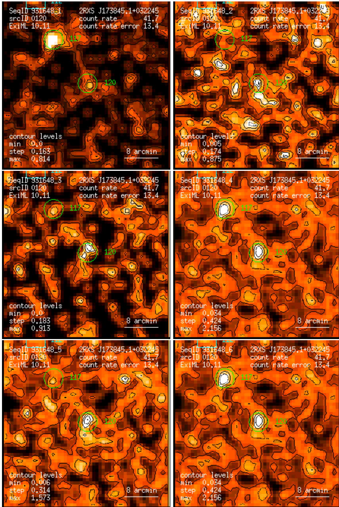
Figure 120: RASS 931648: detection 0120: band rate images, Gaussian filter: (1) PSPC channels 11 – 41, (2) 52 – 90, (3) 91 – 201, (4) 11 – 235, (5) 52 – 201, (6) 11 – 201. Broad band rates in counts/ks. Band rate contour levels in counts/ks/arcmin 2 .
