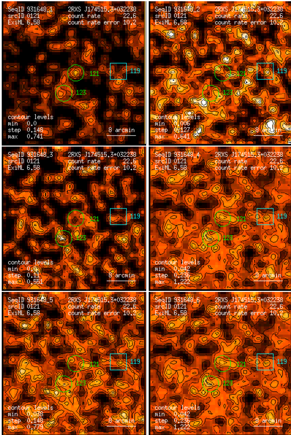
Figure 121: RASS 931648: detection 0121: band rate images, Gaussian filter: (1) PSPC channels 11 – 41, (2) 52 – 90, (3) 91 – 201, (4) 11 – 235, (5) 52 – 201, (6) 11 – 201. Broad band rates in counts/ks. Band rate contour levels in counts/ks/arcmin 2 .
