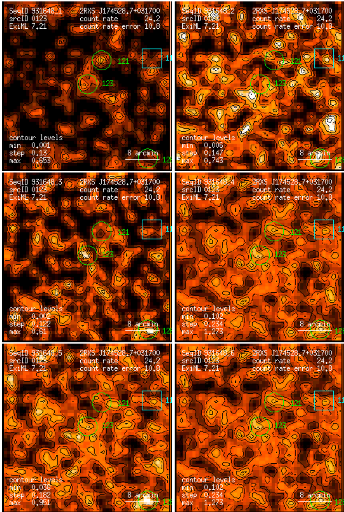
Figure 123: RASS 931648: detection 0123: band rate images, Gaussian filter: (1) PSPC channels 11 – 41, (2) 52 – 90, (3) 91 – 201, (4) 11 – 235, (5) 52 – 201, (6) 11 – 201. Broad band rates in counts/ks. Band rate contour levels in counts/ks/arcmin 2 .
