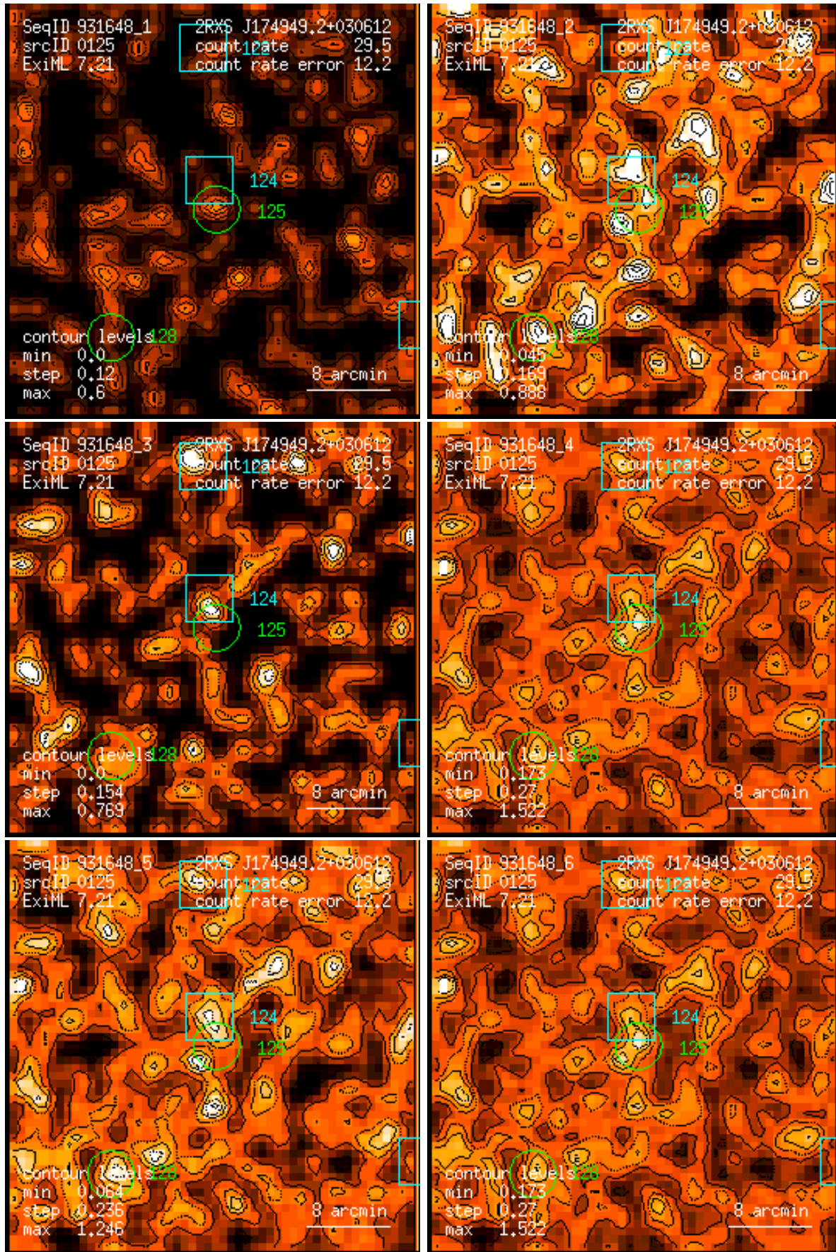
Figure 125: RASS 931648: detection 0125: band rate images, Gaussian filter: (1) PSPC channels 11 – 41, (2) 52 – 90, (3) 91 – 201, (4) 11 – 235, (5) 52 – 201, (6) 11 – 201. Broad band rates in counts/ks. Band rate contour levels in counts/ks/arcmin 2 .
