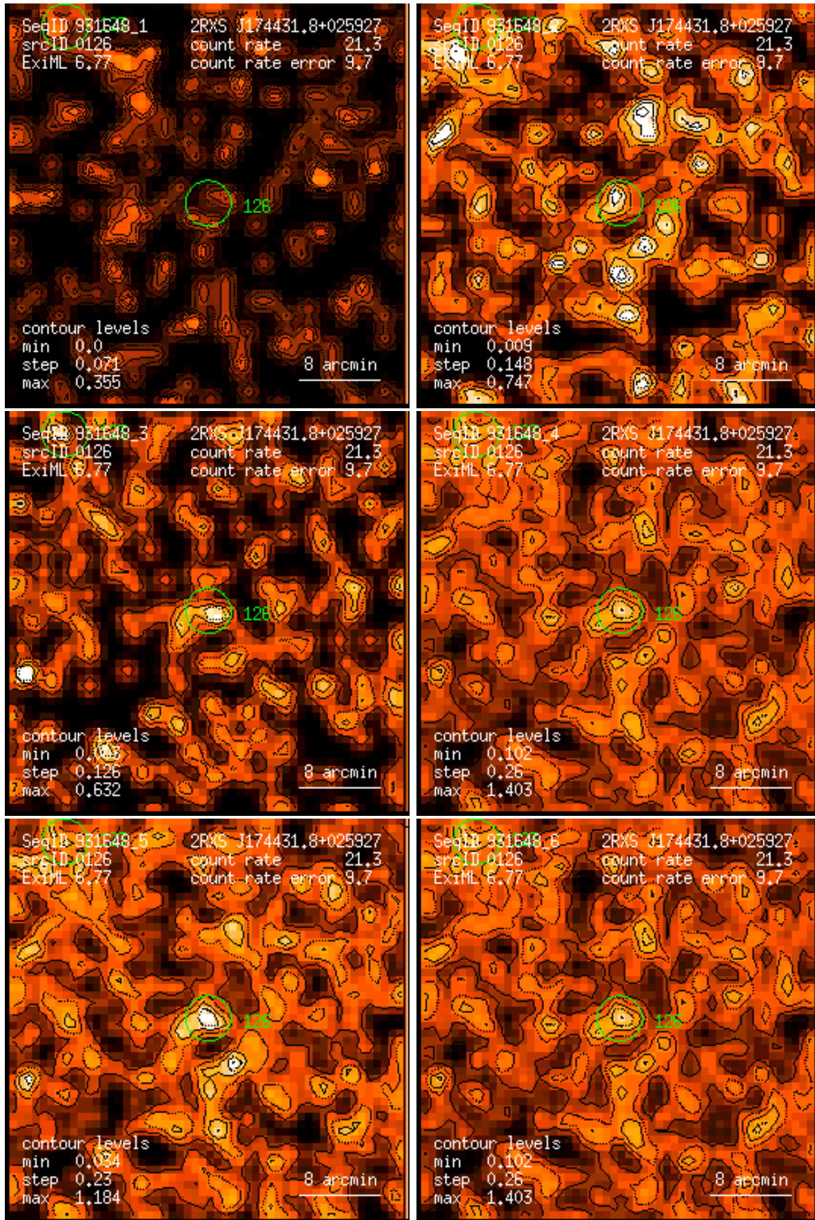
Figure 126: RASS 931648: detection 0126: band rate images, Gaussian filter: (1) PSPC channels 11 – 41, (2) 52 – 90, (3) 91 – 201, (4) 11 – 235, (5) 52 – 201, (6) 11 – 201. Broad band rates in counts/ks. Band rate contour levels in counts/ks/arcmin 2 .
