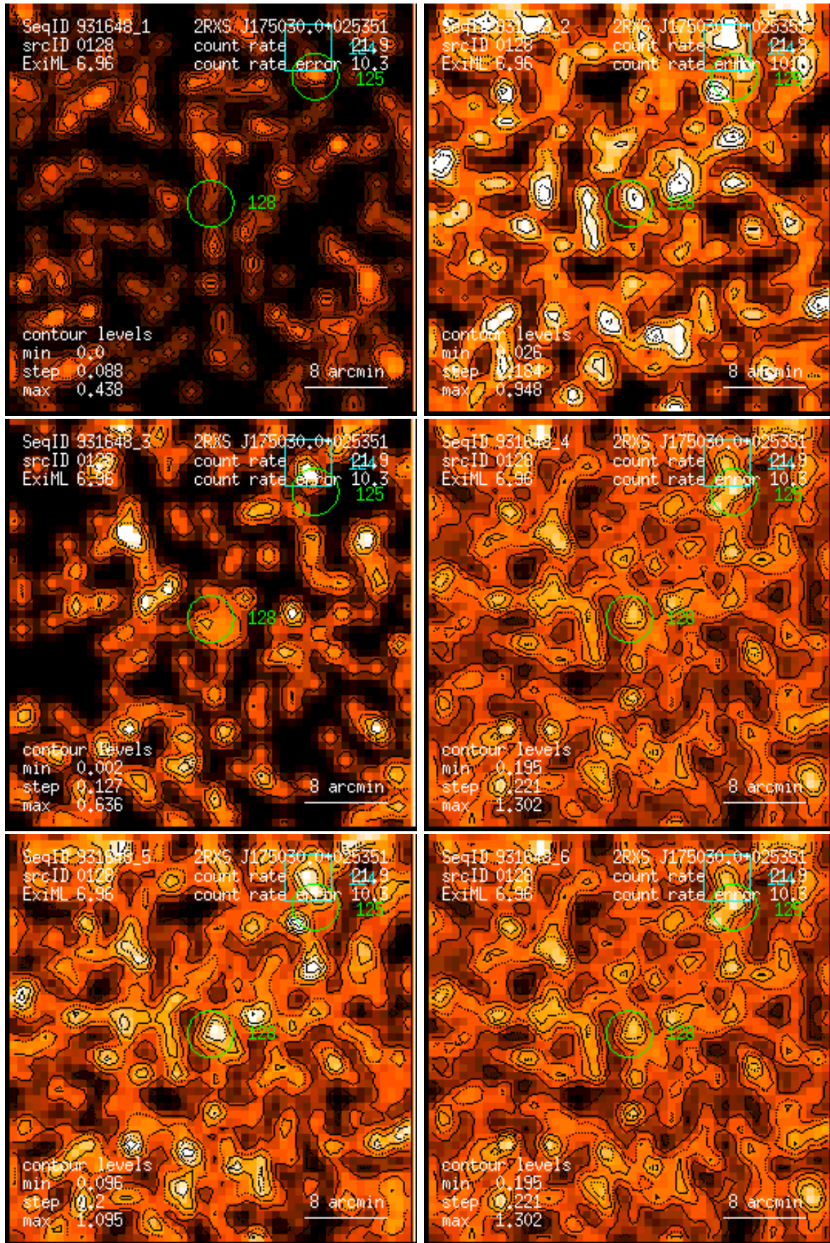
Figure 128: RASS 931648: detection 0128: band rate images, Gaussian filter: (1) PSPC channels 11 – 41, (2) 52 – 90, (3) 91 – 201, (4) 11 – 235, (5) 52 – 201, (6) 11 – 201. Broad band rates in counts/ks. Band rate contour levels in counts/ks/arcmin 2 .
