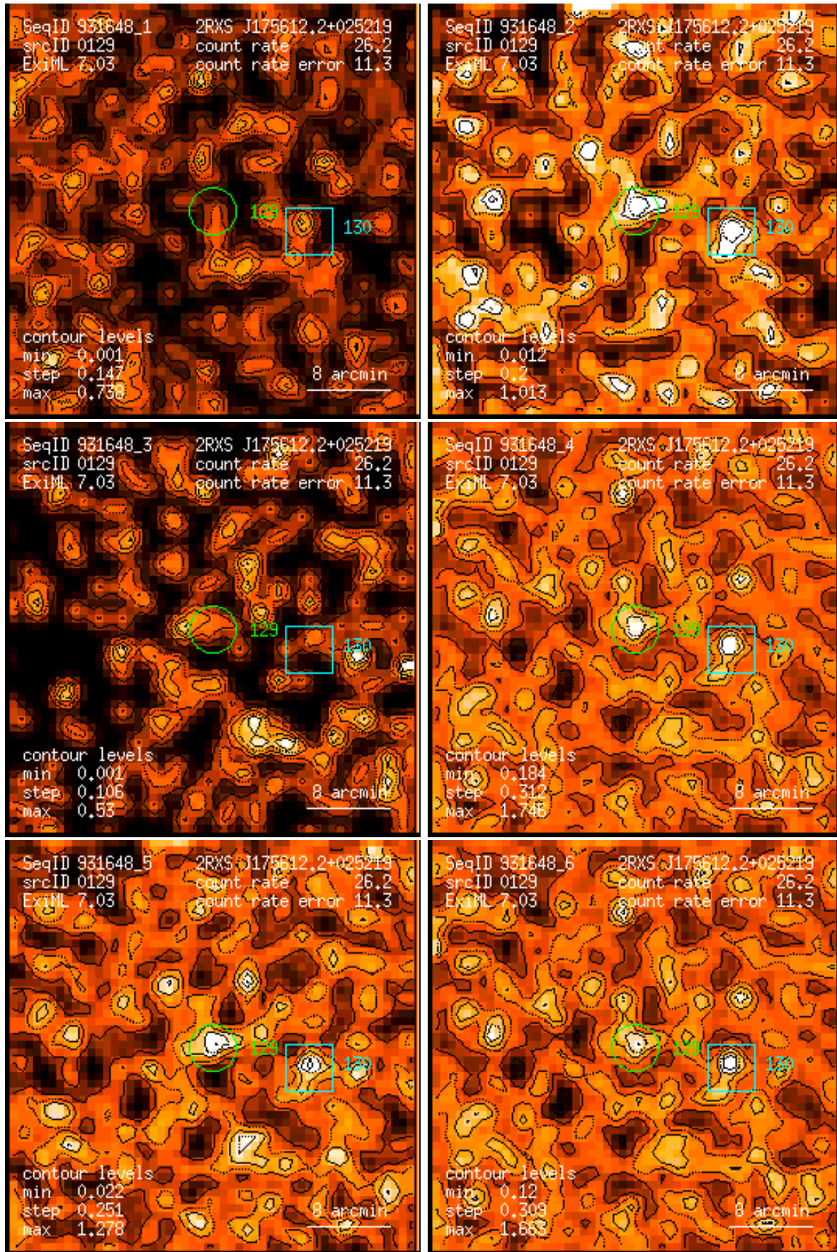
Figure 129: RASS 931648: detection 0129: band rate images, Gaussian filter: (1) PSPC channels 11 – 41, (2) 52 – 90, (3) 91 – 201, (4) 11 – 235, (5) 52 – 201, (6) 11 – 201. Broad band rates in counts/ks. Band rate contour levels in counts/ks/arcmin 2 .
