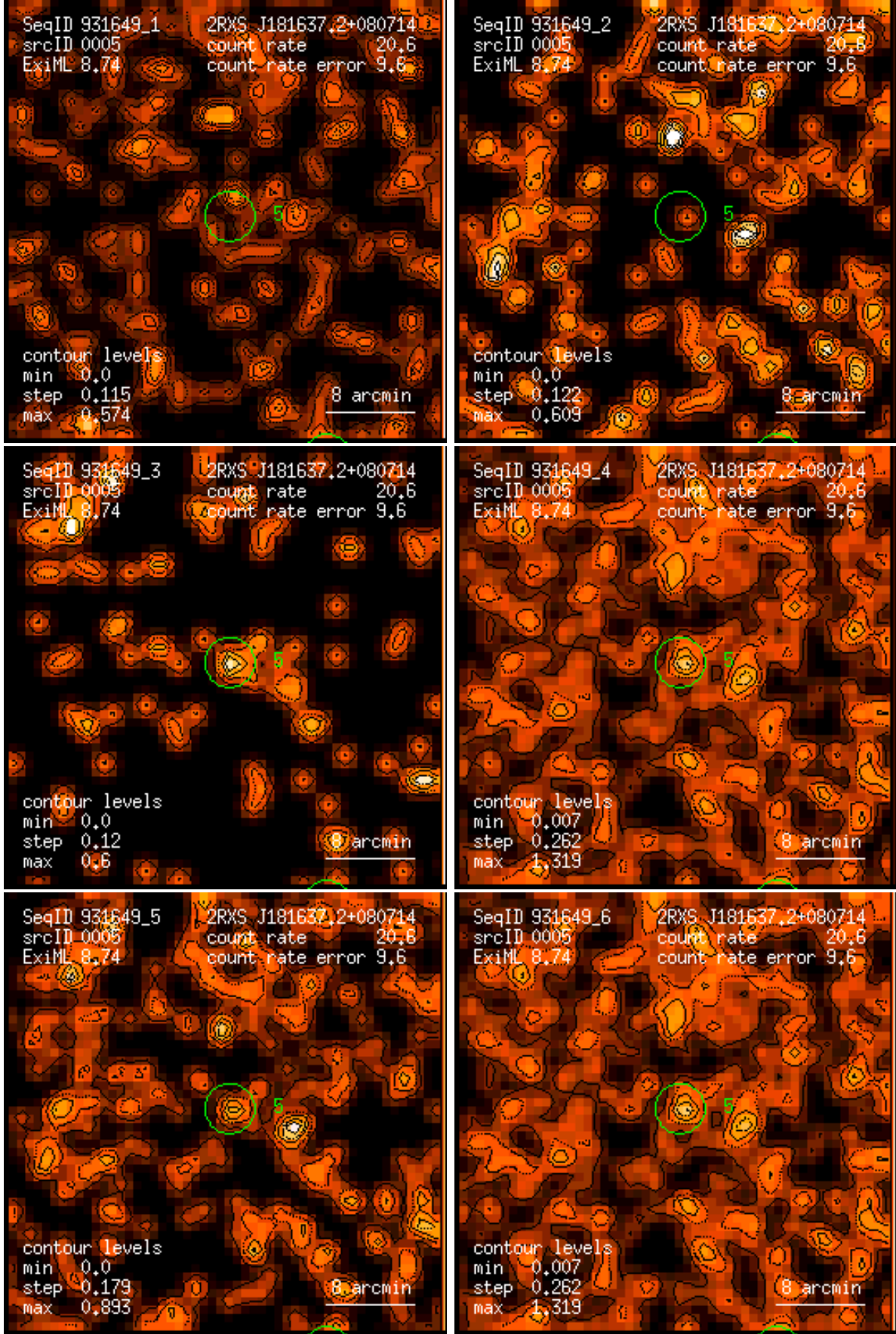
Figure 5: RASS 931649: detection 0005: band rate images, Gaussian filter: (1) PSPC channels 11 – 41, (2) 52 – 90, (3) 91 – 201, (4) 11 – 235, (5) 52 – 201, (6) 11 – 201. Broad band rates in counts/ks. Band rate contour levels in counts/ks/arcmin 2 .
