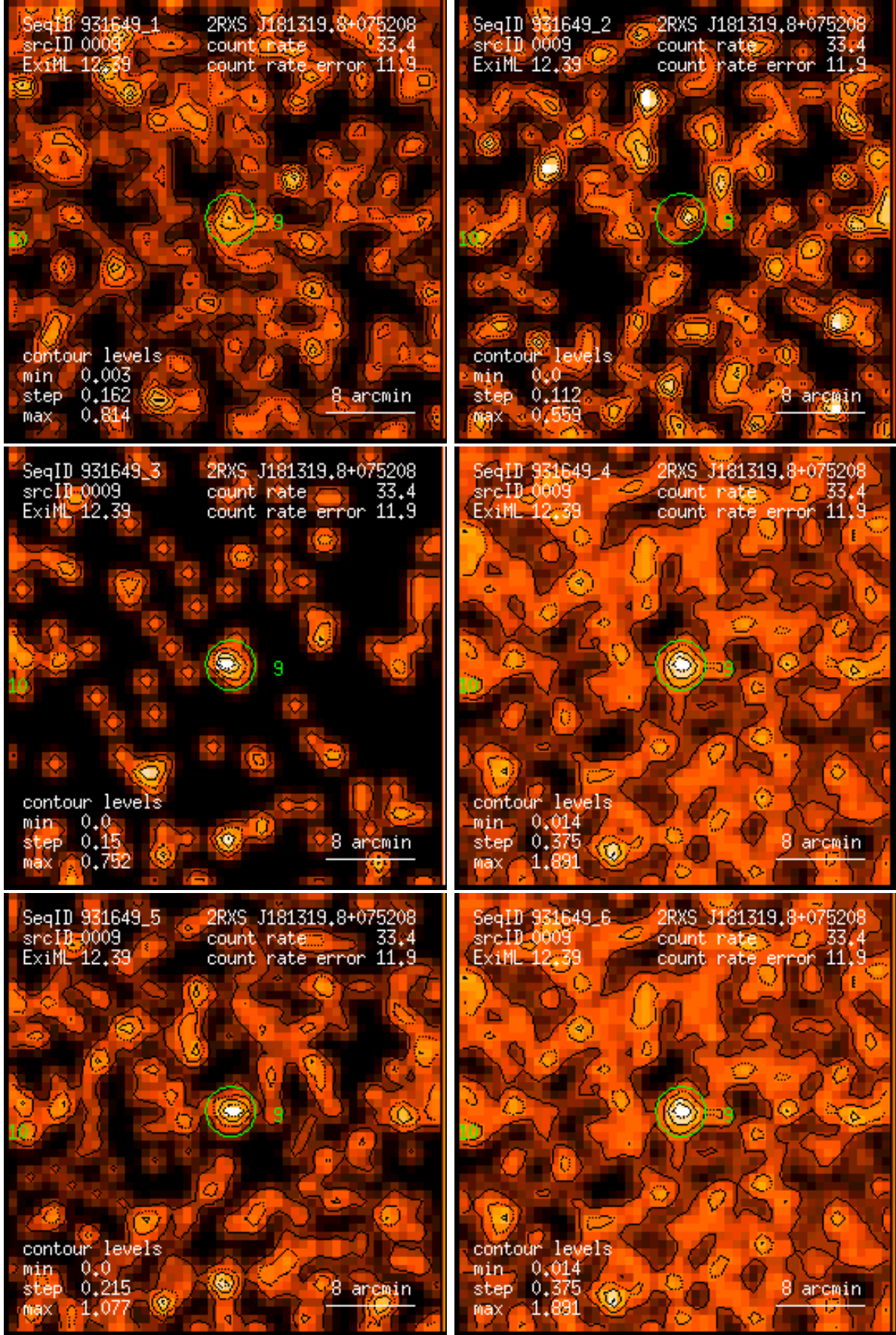
Figure 9: RASS 931649: detection 0009: band rate images, Gaussian filter: (1) PSPC channels 11 – 41, (2) 52 – 90, (3) 91 – 201, (4) 11 – 235, (5) 52 – 201, (6) 11 – 201. Broad band rates in counts/ks. Band rate contour levels in counts/ks/arcmin 2 .
