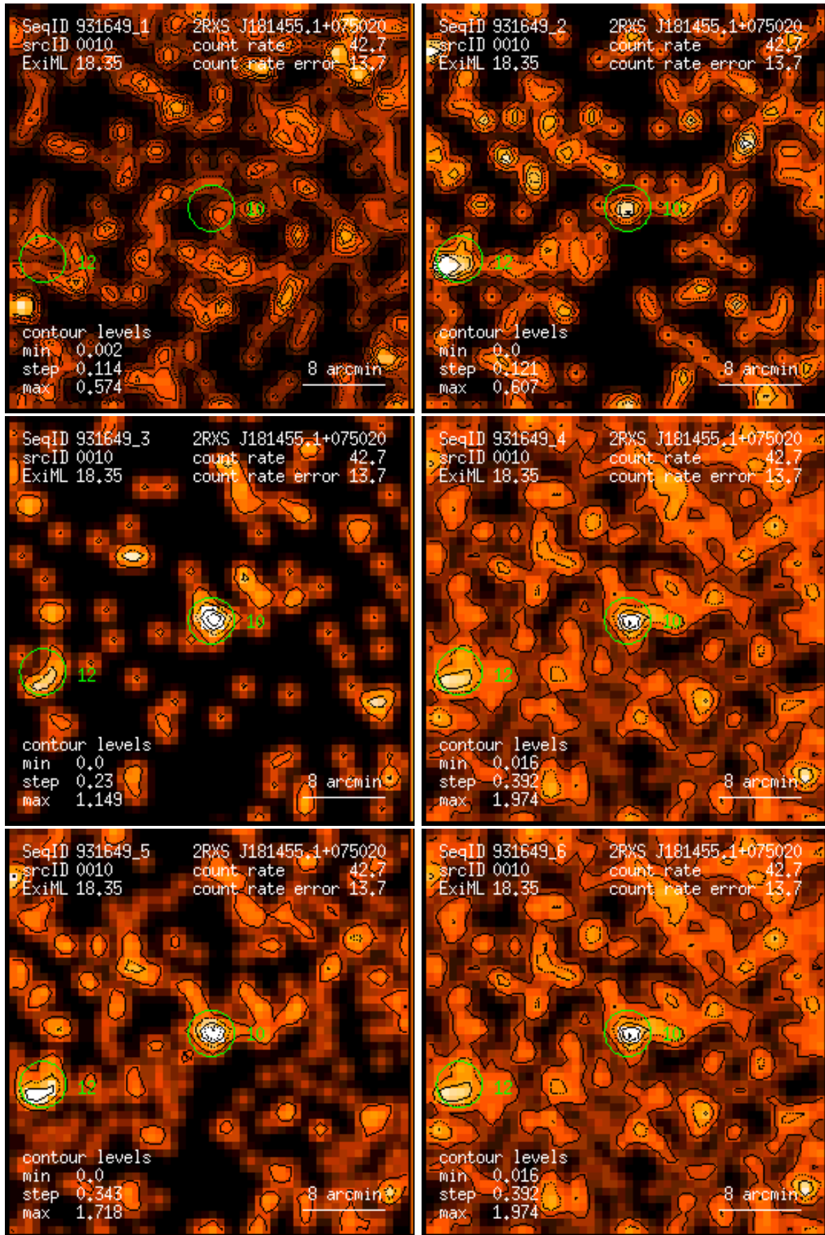
Figure 10: RASS 931649: detection 0010: band rate images, Gaussian filter: (1) PSPC channels 11 – 41, (2) 52 – 90, (3) 91 – 201, (4) 11 – 235, (5) 52 – 201, (6) 11 – 201. Broad band rates in counts/ks. Band rate contour levels in counts/ks/arcmin 2 .
