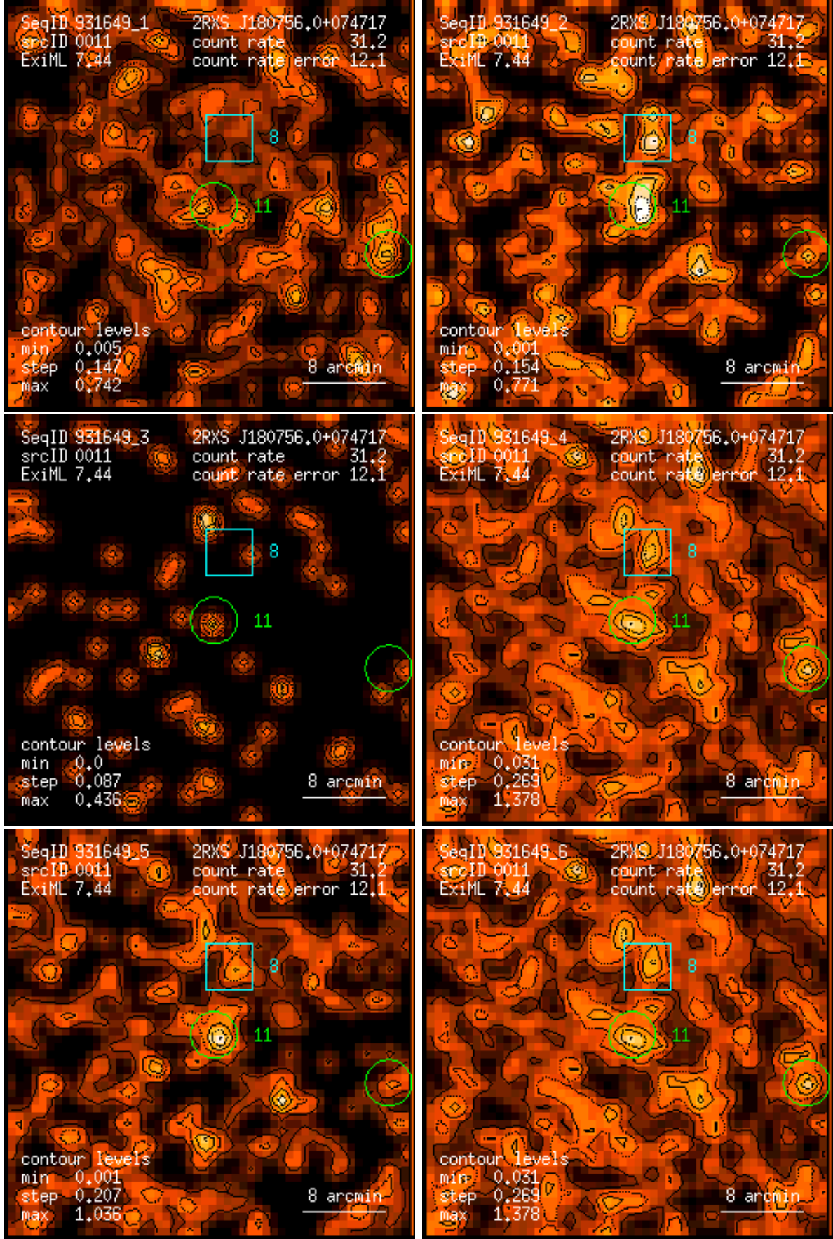
Figure 11: RASS 931649: detection 0011: band rate images, Gaussian filter: (1) PSPC channels 11 – 41, (2) 52 – 90, (3) 91 – 201, (4) 11 – 235, (5) 52 – 201, (6) 11 – 201. Broad band rates in counts/ks. Band rate contour levels in counts/ks/arcmin 2 .
