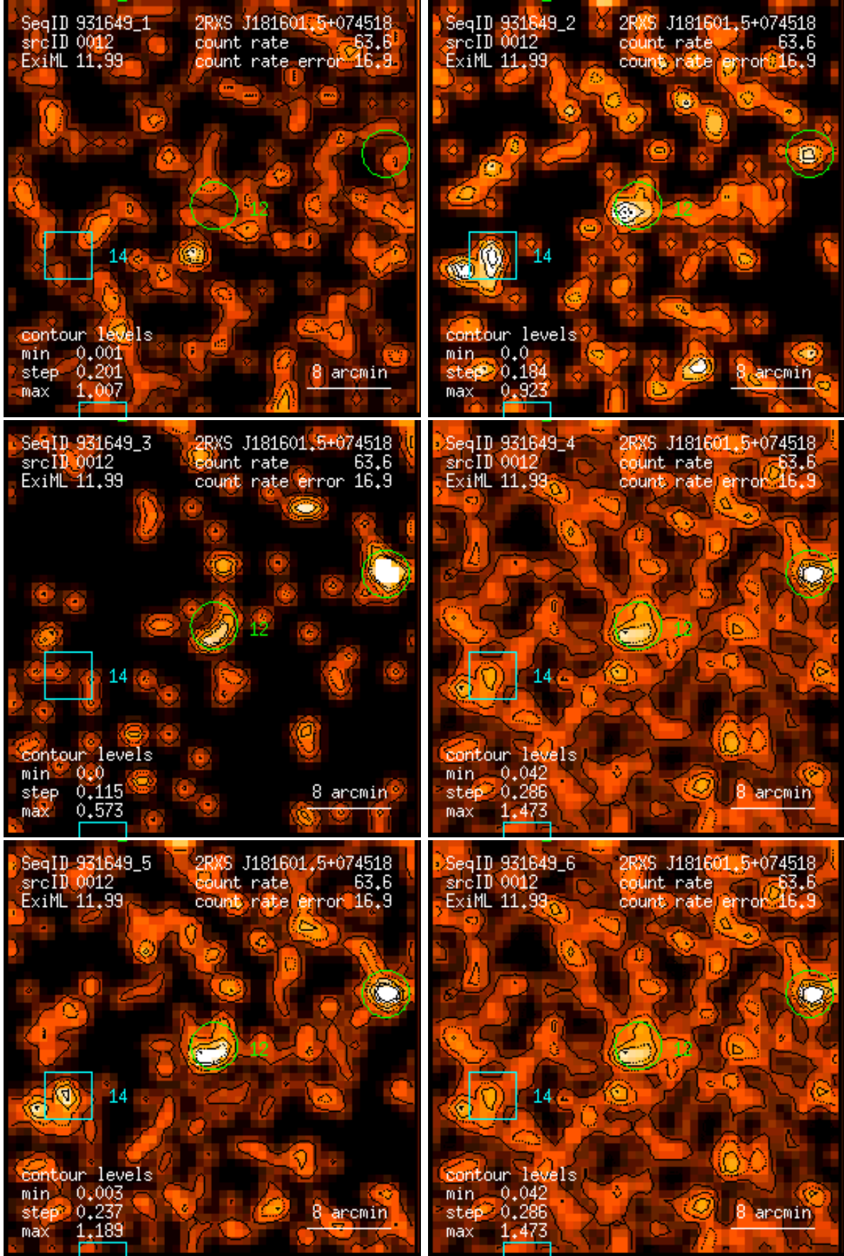
Figure 12: RASS 931649: detection 0012: band rate images, Gaussian filter: (1) PSPC channels 11 – 41, (2) 52 – 90, (3) 91 – 201, (4) 11 – 235, (5) 52 – 201, (6) 11 – 201. Broad band rates in counts/ks. Band rate contour levels in counts/ks/arcmin 2 .
