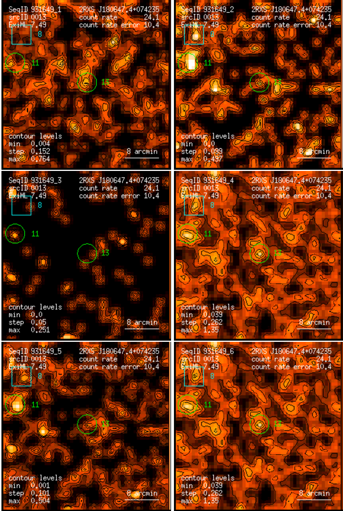
Figure 13: RASS 931649: detection 0013: band rate images, Gaussian filter: (1) PSPC channels 11 – 41, (2) 52 – 90, (3) 91 – 201, (4) 11 – 235, (5) 52 – 201, (6) 11 – 201. Broad band rates in counts/ks. Band rate contour levels in counts/ks/arcmin 2 .
