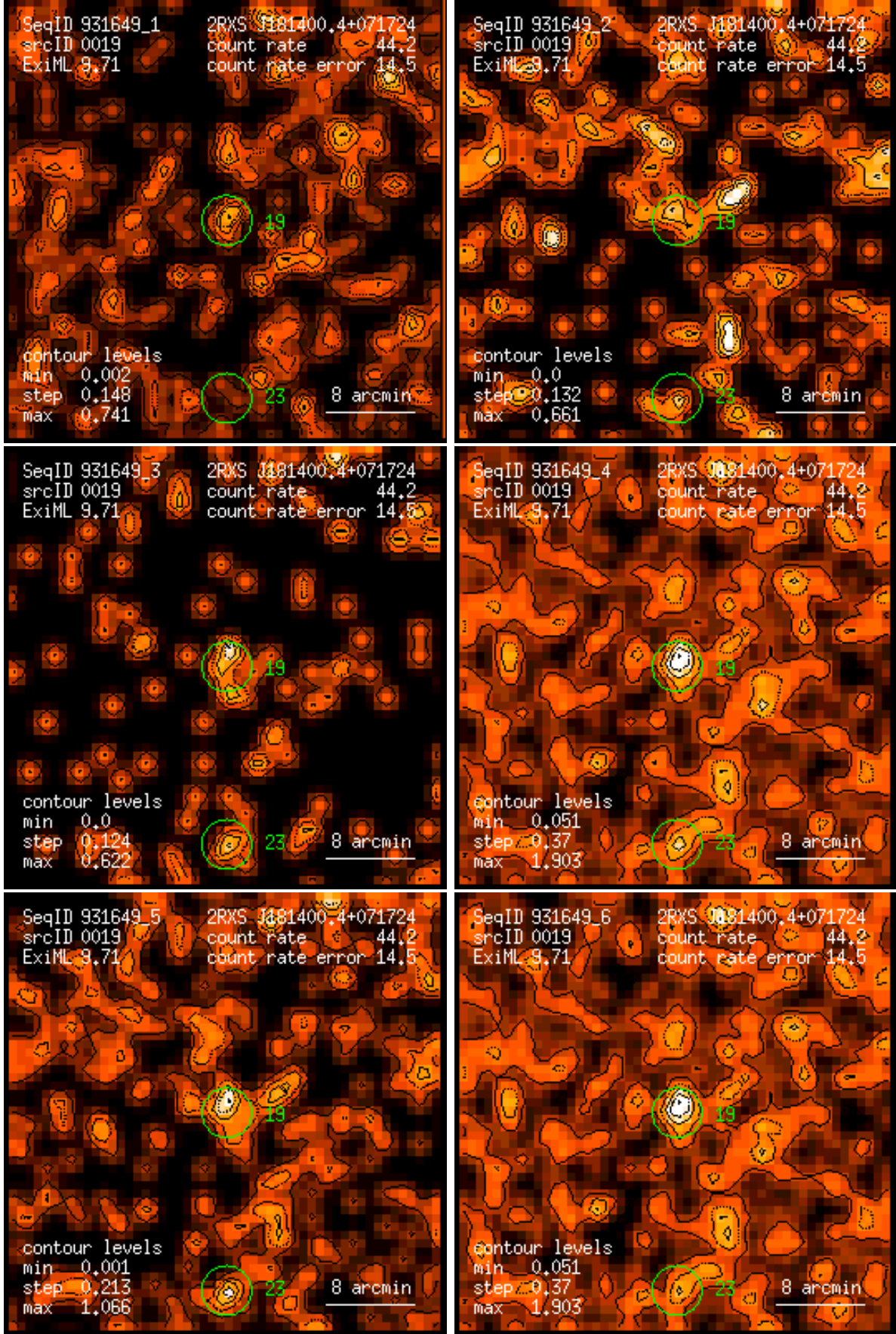
Figure 19: RASS 931649: detection 0019: band rate images, Gaussian filter: (1) PSPC channels 11 – 41, (2) 52 – 90, (3) 91 – 201, (4) 11 – 235, (5) 52 – 201, (6) 11 – 201. Broad band rates in counts/ks. Band rate contour levels in counts/ks/arcmin 2 .
