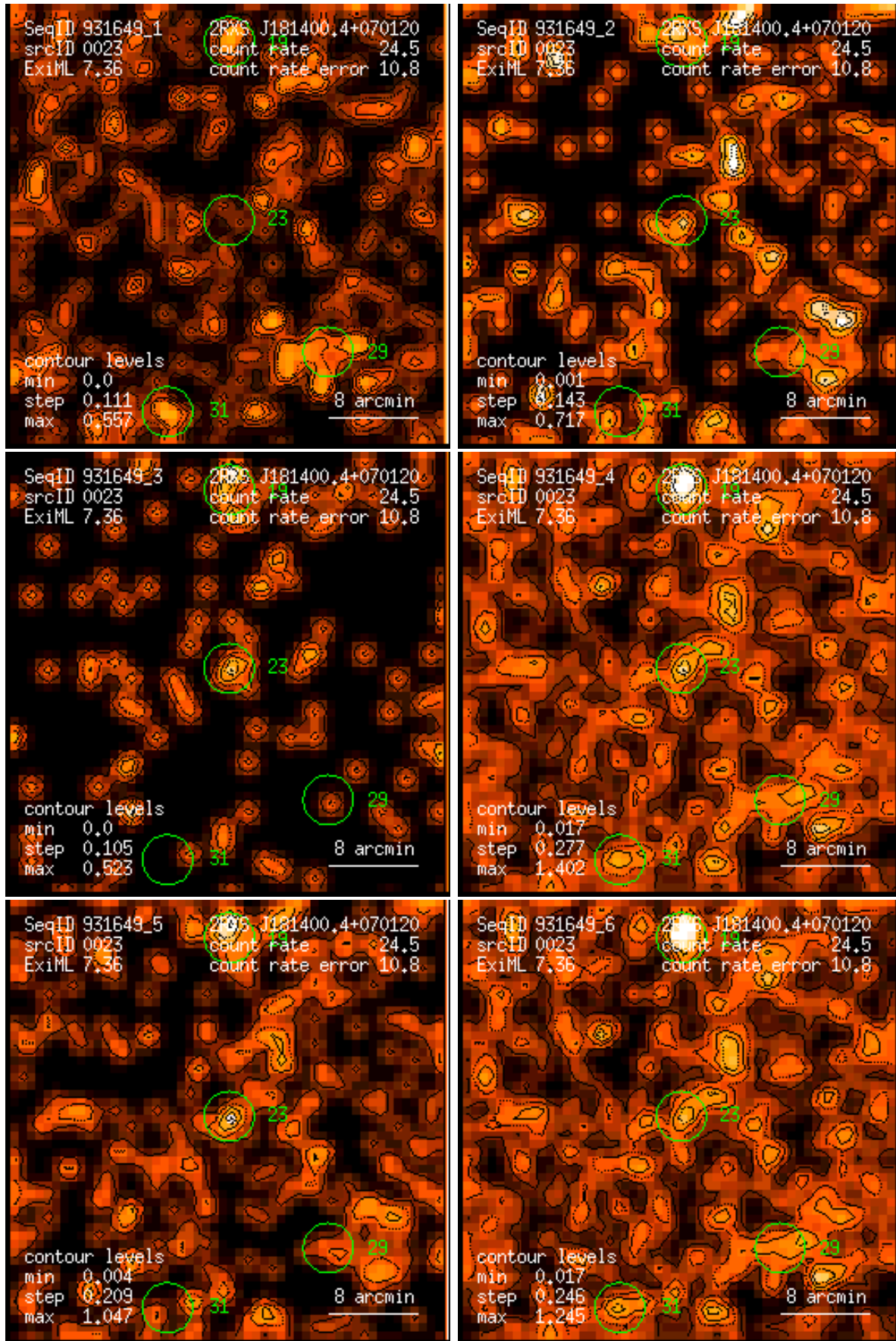
Figure 23: RASS 931649: detection 0023: band rate images, Gaussian filter: (1) PSPC channels 11 – 41, (2) 52 – 90, (3) 91 – 201, (4) 11 – 235, (5) 52 – 201, (6) 11 – 201. Broad band rates in counts/ks. Band rate contour levels in counts/ks/arcmin 2 .
