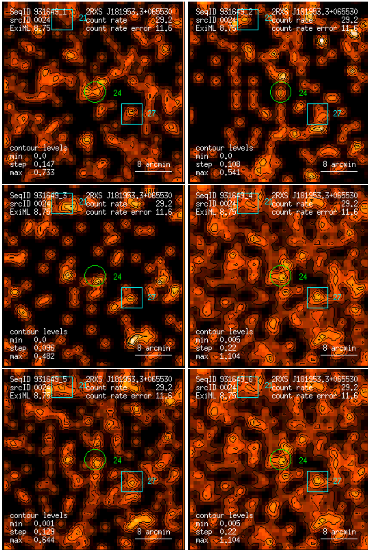
Figure 24: RASS 931649: detection 0024: band rate images, Gaussian filter: (1) PSPC channels 11 – 41, (2) 52 – 90, (3) 91 – 201, (4) 11 – 235, (5) 52 – 201, (6) 11 – 201. Broad band rates in counts/ks. Band rate contour levels in counts/ks/arcmin 2 .
