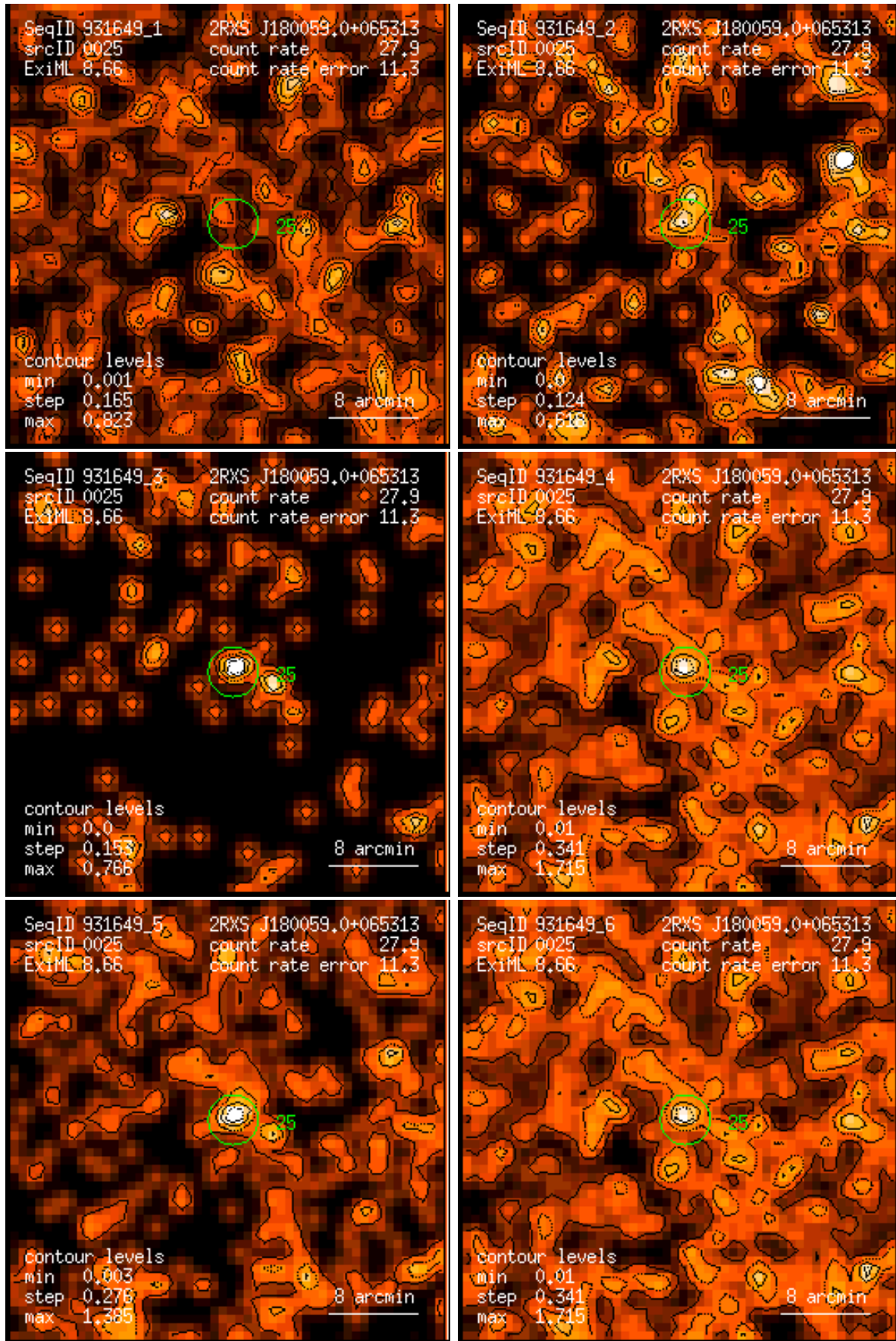
Figure 25: RASS 931649: detection 0025: band rate images, Gaussian filter: (1) PSPC channels 11 – 41, (2) 52 – 90, (3) 91 – 201, (4) 11 – 235, (5) 52 – 201, (6) 11 – 201. Broad band rates in counts/ks. Band rate contour levels in counts/ks/arcmin 2 .
