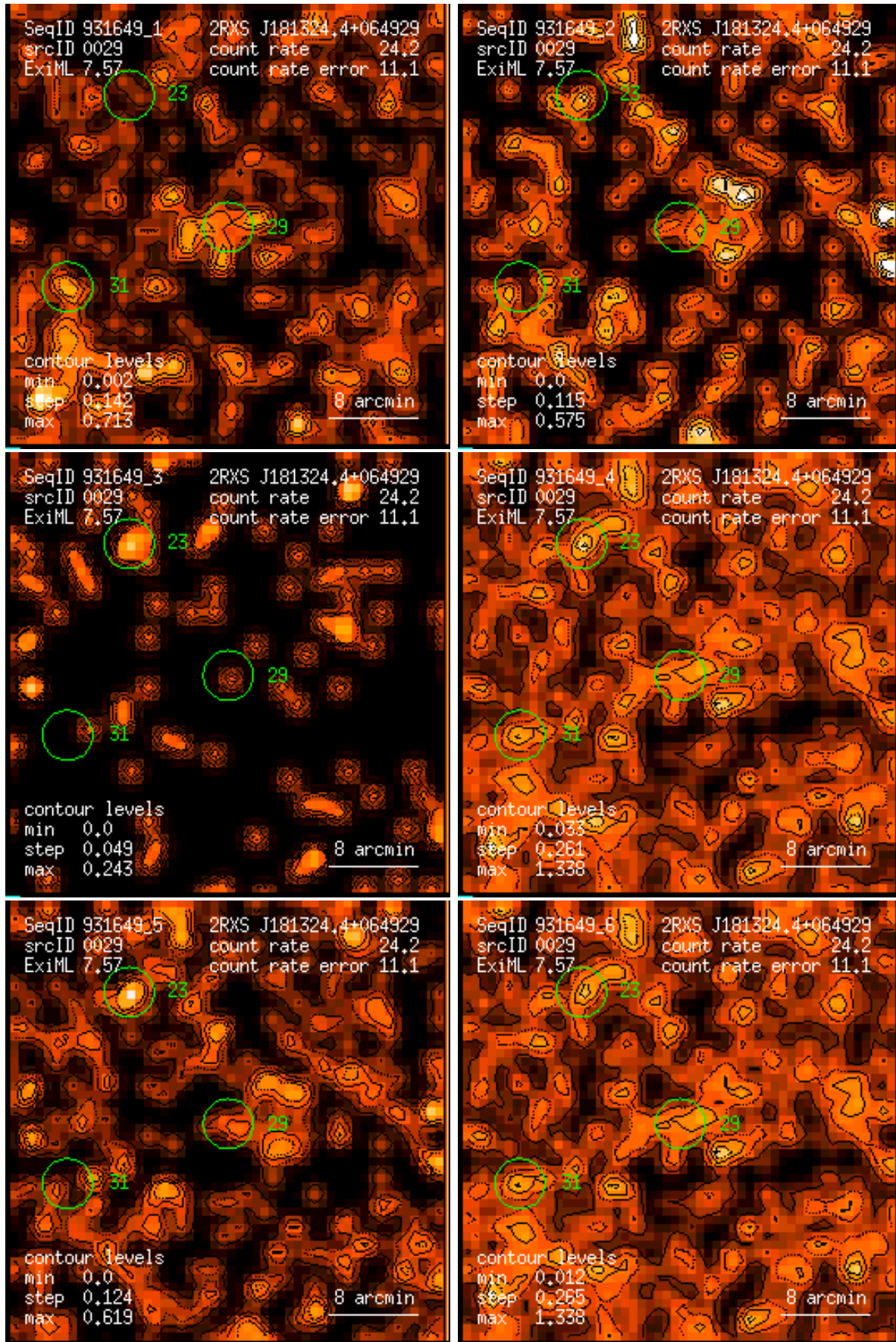
Figure 29: RASS 931649: detection 0029: band rate images, Gaussian filter: (1) PSPC channels 11 – 41, (2) 52 – 90, (3) 91 – 201, (4) 11 – 235, (5) 52 – 201, (6) 11 – 201. Broad band rates in counts/ks. Band rate contour levels in counts/ks/arcmin 2 .
