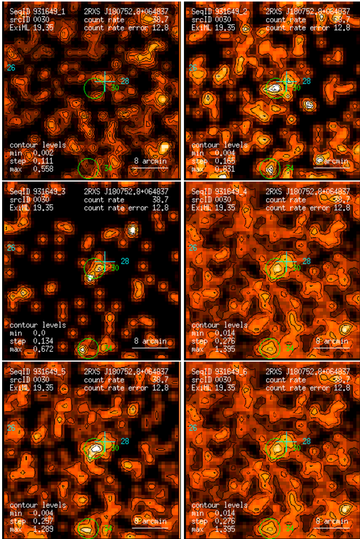
Figure 30: RASS 931649: detection 0030: band rate images, Gaussian filter: (1) PSPC channels 11 – 41, (2) 52 – 90, (3) 91 – 201, (4) 11 – 235, (5) 52 – 201, (6) 11 – 201. Broad band rates in counts/ks. Band rate contour levels in counts/ks/arcmin 2 .
