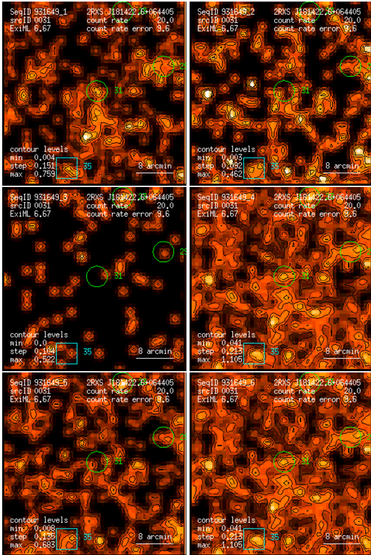
Figure 31: RASS 931649: detection 0031: band rate images, Gaussian filter: (1) PSPC channels 11 – 41, (2) 52 – 90, (3) 91 – 201, (4) 11 – 235, (5) 52 – 201, (6) 11 – 201. Broad band rates in counts/ks. Band rate contour levels in counts/ks/arcmin 2 .
