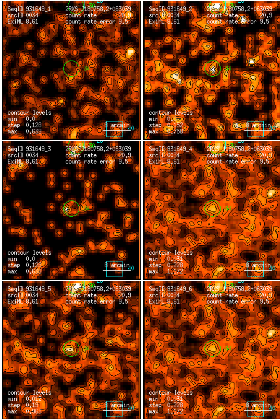
Figure 34: RASS 931649: detection 0034: band rate images, Gaussian filter: (1) PSPC channels 11 – 41, (2) 52 – 90, (3) 91 – 201, (4) 11 – 235, (5) 52 – 201, (6) 11 – 201. Broad band rates in counts/ks. Band rate contour levels in counts/ks/arcmin 2 .
